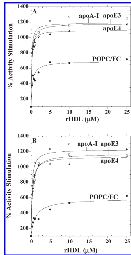
FIGURE 2: Stimulation of the enzymatic activity of PON1 by HDL. Delipidated rePON1 was incubated with increasing concentrations of different rHDLs at rHDL/rePON1 molar ratios of 2.5–250. The initial rates of esterase and lactonase hydrolysis were measured with phenyl acetate (A) and TBBL (B), respectively (using substrate concentrations of 1 mM). Activity is presented as the percentage of the initial activity relative to the delipidated enzyme assigned as 100%. Data were fitted to Langmuir saturation curve, and the activation factor ( V_{max} ) and apparent K_d values were derived (13). Each curve represents the mean of at least three independent experiments. Standard deviations were less than 10% of the parameter values.
