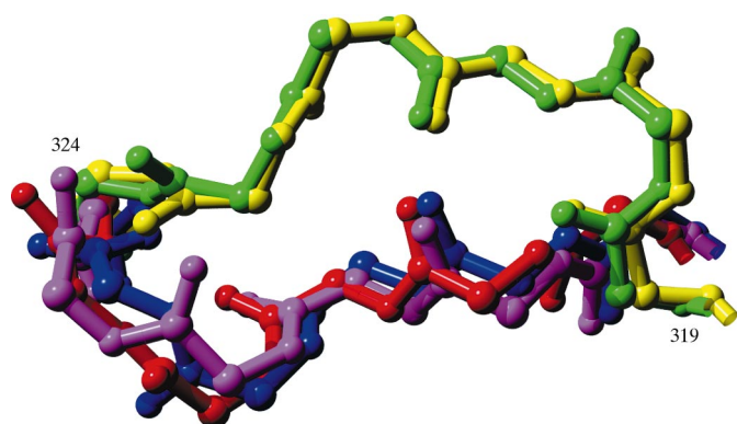
Figure 5 Overlay of the loop 319(310)–324(317) in three AChE–FAS-II complexes and two AChE apo structures: magenta, hAChE–FAS-II; red, mAChE–FAS-II; blue, mAChE (chain A); yellow, TcAChE–FAS-II; green, TcAChE.
