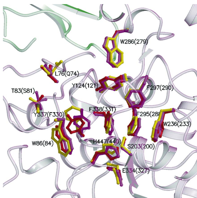
Figure 6 Comparison of the key residues within the active-site gorge in the three complex structures: magenta, hAChE–FAS-II; red, mAChE–FAS-II; yellow, TcAChE–FAS-II. The grey ribbon denotes the hAChE backbone and the green ribbon the FAS-II backbone.
