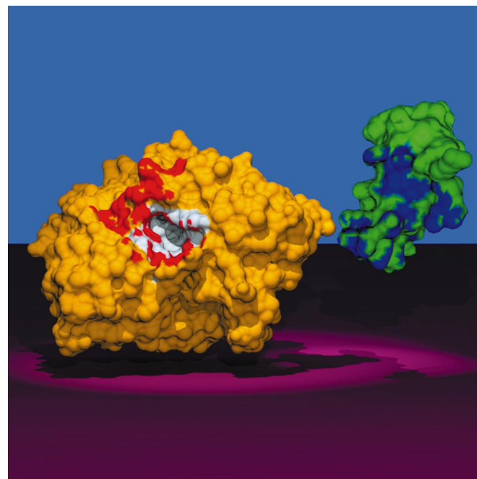
Figure 7 4.0 Å contact footprint between AChE and FAS-II. On the left, molecular surface of hAChE in yellow, with atoms \leq 4.0 Å from FAS-II rendered in red and atoms lining the active-site gorge rendered in grey. On the right, molecular surface of FAS-II in green, with atoms \leq 4.0 Å from hAChE atoms rendered in blue.
