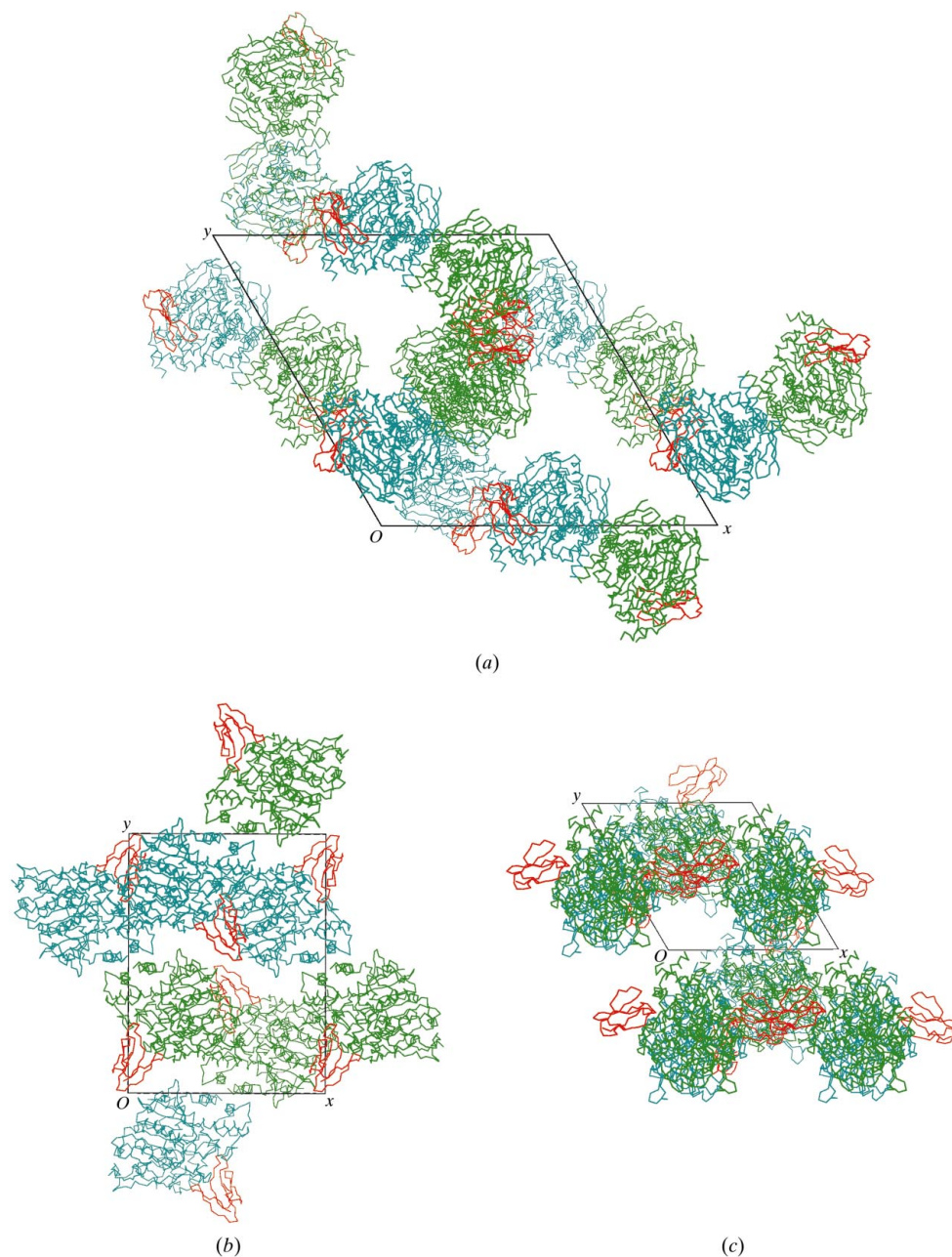
Figure 4 Schematic comparison of packing diagrams of AChE–FAS-II complexes, looking down the z axis with the monomers of the AChE dimers shown in green and blue and FAS-II shown in red: (a) hAChE–FAS-II; (b) TcAChE–FAS-II; (c) mAChE–FAS-II.
