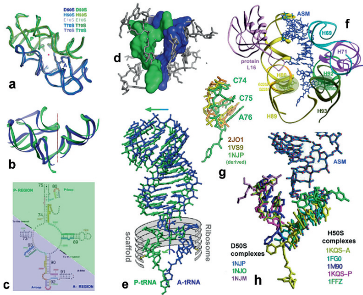
Figure 2. The symmetrical region and peptide bond formation. (a–c). The universal symmetrical region backbone fold. In all structures, the A- and P- sub-regions are shown in blue and green, respectively. The imaginary symmetry axis is shown in red. (a) Superposition of fold of the 180 nucleotides comprising the symmetry region in all known structures, shown as ribbons. The two pseudo-symmetrical sub-regions, containing the A- and the P-sites, are shown in blue and green respectively. The imaginary axis relating the two halves of the symmetrical region is shown as a red rod (or its cross-section). The center of the PTC lies roughly on this axis. (b) Superposition of the backbones of the rRNA comprising the A- and P- sub-regions of the symmetrical region, as obtained by a 180° rotation around the imaginary symmetry axis, indicating the level of the ribosomal internal symmetry. (c) Two-dimensional representation of the 23S rRNA segment that belongs to the symmetrical region. Symmetrical features are shown in identical colors. (d) Superposition of the locations of short substrate analogs used in crystallographic studies together with H50S and D50S. The PDB accession codes are indicated. (e) The tRNA translocation motion, comprising a synchronized sideways shift, performed as part of the overall mRNA/tRNA sideways translocation (in the direction of the horizontal arrow), and the rotatory motion of the A-tRNA 3' end along a path confined by the PTC grey walls (shown here as ribs). The A-site tRNA and the derived 3' end of the P-site tRNA are shown in blue and green (respectively). The direction of the rotatory motions is indicated by a blue-green curved arrow, the imaginary twofold symmetry axis is red, and the approximated positions of the symmetrical basepairs [23, 32, 39, 40] are shown in yellow. (f) Superposition of the derived P-site CCA (from ASM 3' end by the rotatory motion) on the crystallographically determined locations of the P-site CCA in crystals of 70S complexes [11, 12]. The PDB accession codes are indicated.
