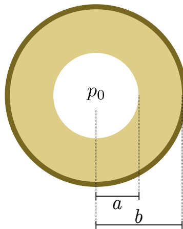
Figure 1: Reinforced thick Wall cylinder
