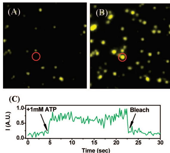
Figure 3. Activity of the optical switch in labeled SR1WC molecules deposited on a glass surface, monitored at the single molecule level. Changes in fluorescence after addition of (A) buffer only and (B) 1 mM ATP. (C) Temporal trajectory of the molecule marked with a red circle in (A) and (B).
