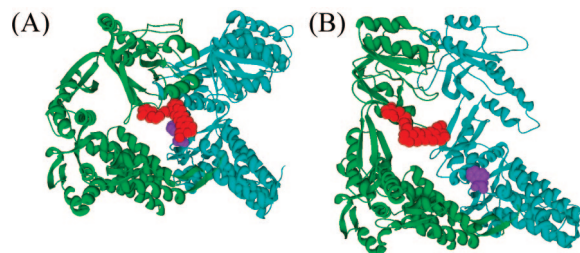
Figure 1. The optical switch in single-ring GroEL (SR1) molecules. (A) The fluorescence of the oxazine dye at position 327 (in red) is quenched by Trp44 (in violet) in the T conformation of GroEL. (B) In the R' conformation, the quenching is removed. The structures shown in A and B are those of two adjacent subunits in the trans and cis rings, respectively, of the GroEL-GroES-ADP 7 complex (9).
