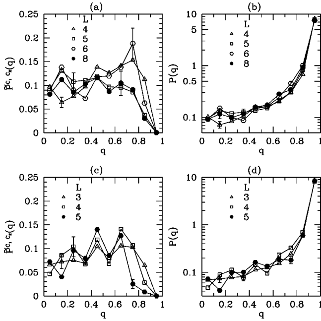
FIG. 15. (a) The partial distribution \tilde{P}^{C_1 C_2}(q) for D=3 , L=4,5,6,8 . It is normalized so that 2\int_0^1 \tilde{P}^{C_1 C_2}(q) is its weight in the total P(q) . For clarity only a few representative error bars are shown. (b) The distribution P(q) for the same systems as in (a). (c) \tilde{P}^{C_1 C_2}(q) as in (a) but for D=4 , L=3,4,5 . (d) P(q) for the same systems as in (c).
