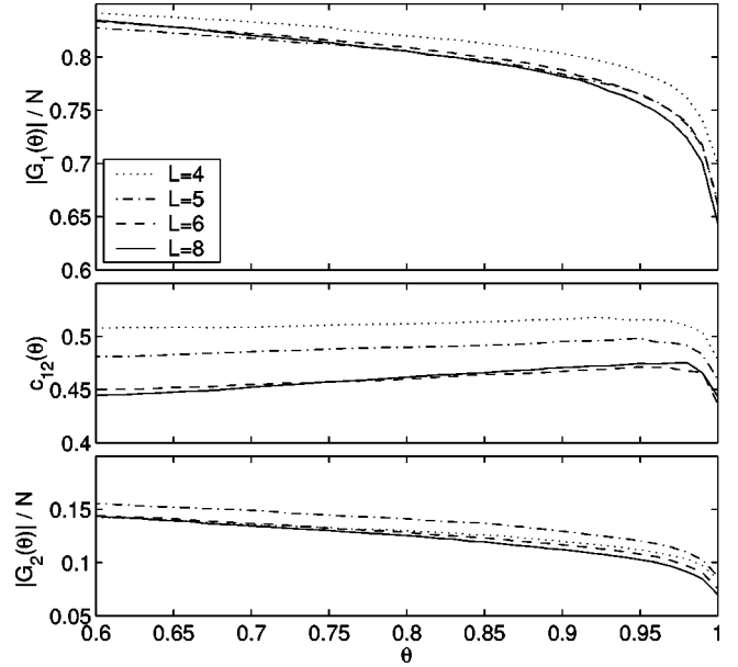
FIG. 7. The normalized sizes of the two largest spin domains, \mathcal{G}_1(\theta)/N and \mathcal{G}_2(\theta)/N and their correlation \bar{c}_{12} , defined in Eq. (25), as a function of the threshold \theta for D=3 , T=0.2 .
