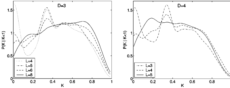
FIG. 17. The distribution P(K|K<1) of K_{\mu\nu\rho} , for \mu \in C_2 , \nu \in C_{1a} , and \rho \in C_{1b} . All systems are sampled at T=0.2 .
