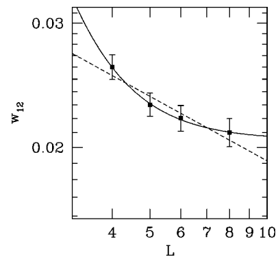
FIG. 6. A log-log plot of w_{12} against L for T=0.2 and D=3 . The solid line is the best least squares fit to Eq. (17), while the dashed line is the best fit with the additional assumption that w_\infty = 0 .
