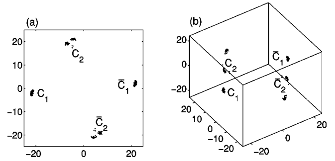
FIG. 5. Principal component analysis of a sample of M=500 \times 2 states of a specific realization of \{J\} in 3D with N=8^3 spins at T=0.2 . Each point represents a state \mathbf{S}^\mu . The coordinates are projections onto eigenvectors \mathbf{e}_i , corresponding to the largest eigenvalues of the correlation matrix in Eq. (11). We show in (a) projections onto two eigenvectors, corresponding to the largest and next-largest eigenvalues of the correlation matrix, shown, respectively, on the horizontal and vertical axes. In (b) the three largest eigenvectors are used. The first and second level partitions of the hierarchy are clearly visible and, to some extent, the third level also.
