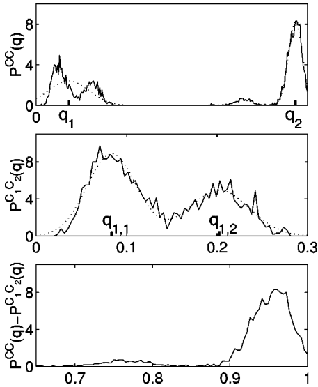
FIG. 16. (Top) The distribution P_J^{CC}(q) for the same 3D realization whose data were presented in Fig. 12. The dotted line is a fit to the sum of two Gaussians (see text). (Middle) The partial distribution P_J^{C_1 C_2}(q) for the same realization. The dotted line represents a fit to the sum of two Gaussians. (Bottom) The difference between the two previous distributions.
