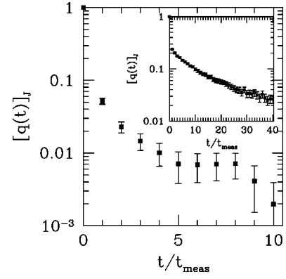
FIG. 2. The main part of the figure shows the correlation between spin configurations, [q(t)]_J , defined in Eq. (5) of the text, in D=3 for L=8, T=0.2 . The horizontal axis represents the number of Monte Carlo sweeps between the two configurations in units of the number of sweeps between individual measurements, t_{\text{meas}} . For comparison, for each set of spins (‘‘replica’’), a total of 250 configurations are generated. The inset shows results for D=3, L=12, T=0.5 , which indicate that correlations between spin configurations are significantly larger than for L=8 .
