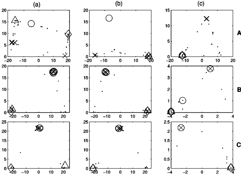
FIG. 13. The two principal components of the 512 spins of three realizations A, B, and C (see text) in 3D. Each point represents a spin i and its coordinates are the projections of \mathbf{S}_i = (S_i^1, S_i^2, \dots, S_i^M) onto the two largest eigenvectors of the matrix R in Eq. (31). The analysis is carried over (a) all states; (b) the states of \mathcal{C}_1 ; and (c) the states of \mathcal{C}_2 . The spins of \mathcal{G}_1 are marked by \diamond ; of \mathcal{G}_2 by \triangle ; of \mathcal{G}_3 by \circ ; and of \mathcal{G}'_3 by \times . Spins that belong to both \mathcal{G}_3 and \mathcal{G}'_3 are marked by \otimes . Spins that do not belong to any of these domains are marked with dots. The lower half of the plane is projected onto the upper half using (x, y) \rightarrow (-x, -y) . Spins in a correlated domain usually have the same values for the two principal components, and they fall on top of each other on the plot. Therefore, in most plots, a correlated domain seems to be represented by a single marker.
