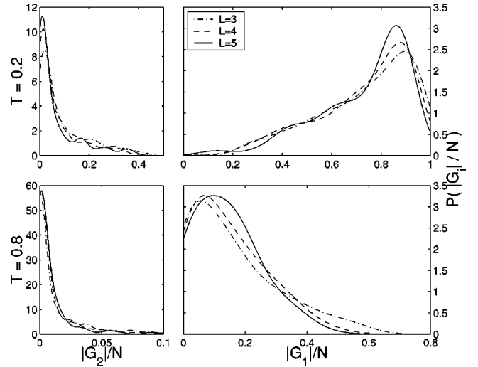
FIG. 10. Size distributions of the spin domains \mathcal{G}_1 and \mathcal{G}_2 for D=4 dimensions at T=0.2, 0.8 . For T=0.2 the distributions seem to converge, despite the small system sizes. For T=0.8 , |\mathcal{G}_2|/N converges to a narrow distribution around zero, and |\mathcal{G}_1|/N does not show convergence yet.
