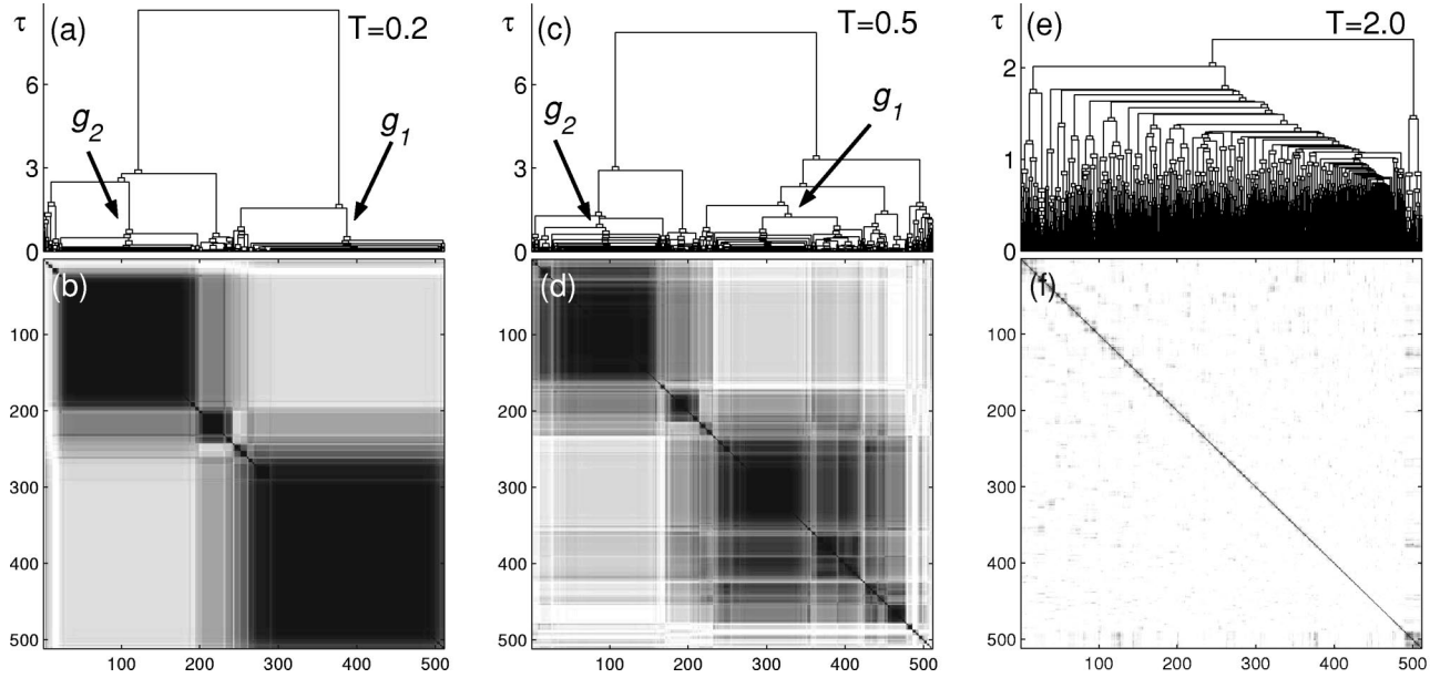
FIG. 11. (a) The spin dendrogram \mathcal{D} for the data of Fig. 4(a) produced by Ward's algorithm. (b) The spin distance matrix d of this realization. The spins are ordered according to their clusters in \mathcal{D} . Darker shades correspond to smaller distances and higher correlations. (c), (d) The same as in (a), (b), for the same realization at T=0.5 . (e), (f) The same as in (a), (b), for the same realization at T=2.0 . The y axis is rescaled to show the dendrogram, which clearly differs from the dendrograms in (a) and (c).
