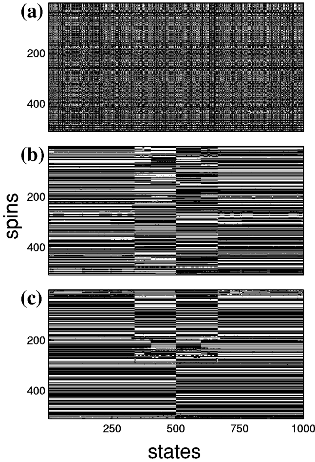
FIG. 4. (a) The original data matrix of 500 \times 2 states \mathbf{S}^\mu , S_i^\mu = \pm 1 , with black/white representing +/- . This 3D sample was generated for a realization of size 8^3 at T=0.2 (the same one as in Fig. 3). The spins are in lexicographic order. (b) The same matrix, with the states ordered according to the dendrogram in Fig. 3. (c) The matrix in (b) with, in addition, the spins ordered according to the spin dendrogram \mathcal{D} in Fig. 11.
