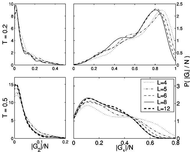
FIG. 9. Size distributions of the spin domains \mathcal{G}_1 and \mathcal{G}_2 for D=3 dimensions at T=0.2, 0.5 . The distributions seem to converge, despite the small system sizes.
