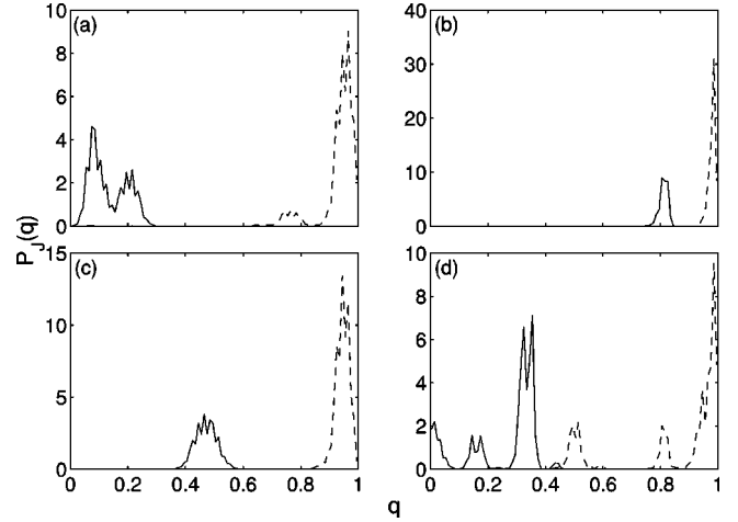
FIG. 14. The distribution P_J(q) for four realizations of \{J\} at T=0.2 in 3D. The distribution in (a) is the same as in the top frame of Fig. 16. The solid line describes P_J^{C_1 C_2}(q) and the dashed line plots the rest of the distribution, P_J(q) - P_J^{C_1 C_2}(q) . The latter contains a large peak at q \approx 1 which is contributed by the distribution P_J^i(q) , or overlaps inside the valleys.
