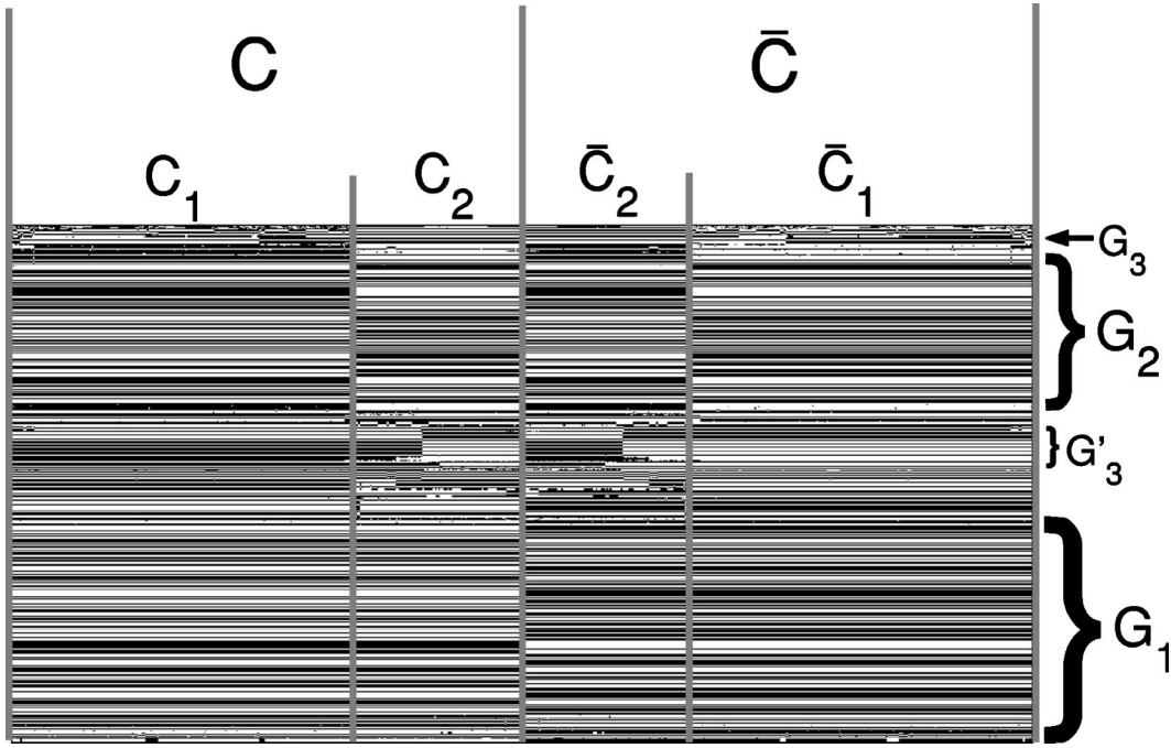
FIG. 12. A redrawing of the ordered data matrix of Fig. 4(c), in order to highlight the state clusters and spin domains discussed in the text. It is for a 3D realization of size N=8^3 at T=0.2 . The columns represent the states \mu and the rows represent the spins i , S_i^\mu = \pm 1 , with black/white representing +/- . The states are ordered according to the dendrogram in Fig. 3, and the spins ordered according to the spin dendrogram \mathcal{D} in Fig. 11. The state clusters and the spin domains are marked (see text).
