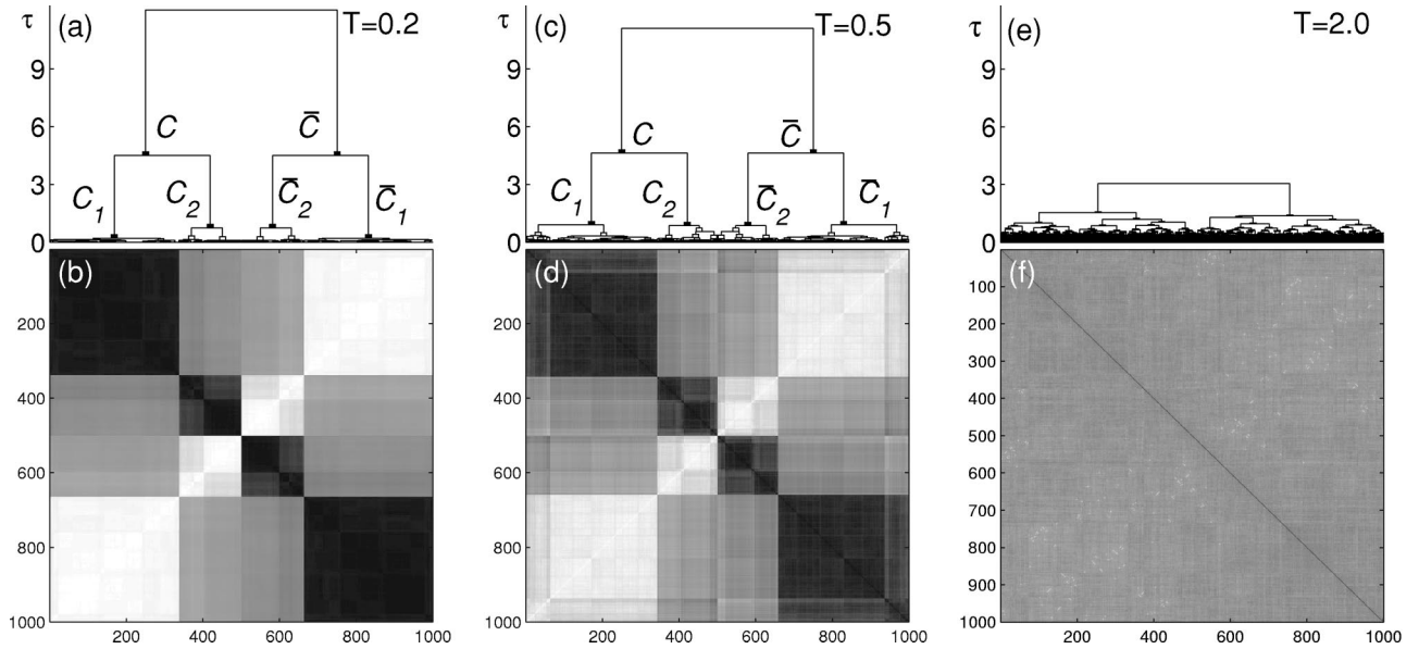
FIG. 3. (a) The dendrogram obtained by clustering the M = 500 \times 2 states of a specific realization in D = 3 of size N = 8^3 at T = 0.2 . The vertical axis describes the value of \tau , defined in Sec. III. (b) The distance matrix of the states used as an input to Ward's algorithm. Darker shades correspond to smaller distances. The states are ordered according to their position on the dendrogram (a). (c), (d) The same as in (a), (b), for the same realization \{J\} , but for an ensemble of states obtained at T = 0.5 . (e), (f) The same as in (a), (b), for the same realization, at T = 2.0 , which is greater than T_c \approx 0.95 . Note that this dendrogram is not symmetric; almost all the distances are close to 0.5, so at each stage of the algorithm there were several possible partitions that gave minimal value to S . In the implementation we used, the algorithm chose a nonsymmetric partition.
