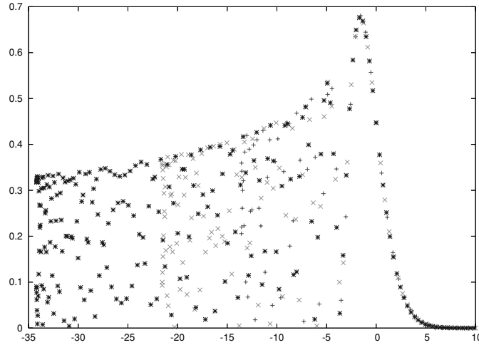
Figure 4. The scaling function f(x) for kR = 50 (red +), kR = 100 (green ×) and for kR = 200 (blue*).
