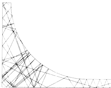
FIG. 1. The elbow system and a typical classical trajectory.
