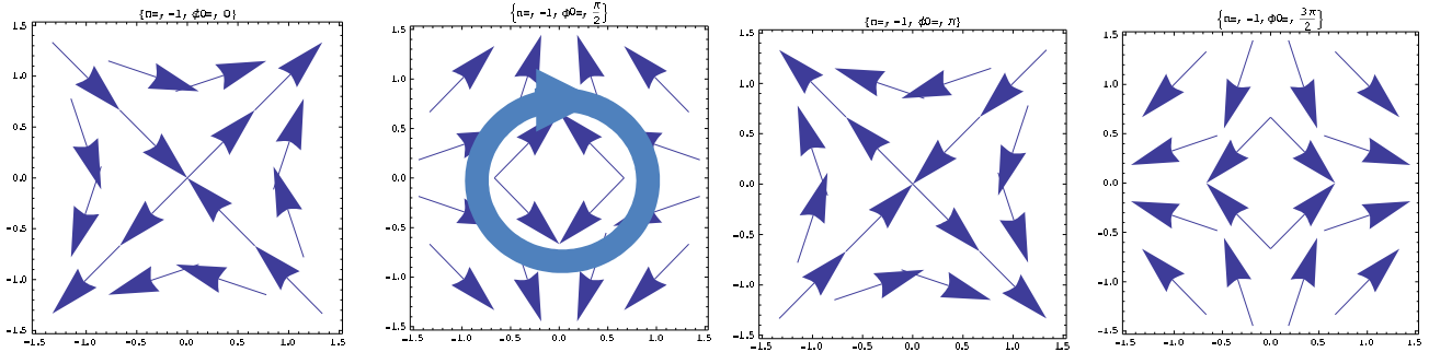
Figure 14: vortex and anti vortex in the spin configuration \psi = \psi_0 e^{i\phi} = S_x - iS_y denoted by arrows in the spin direction and in the velocity \nabla\phi denoted by bold lines
