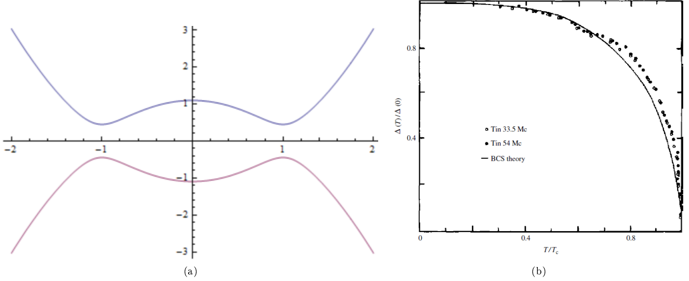
Figure 13: (a) Spectrum of BdG Hamiltonian for \epsilon_{\mathbf{k}} = \frac{k^2}{2m} , and (b) Comparison between BCS gap equation and experimental data.
