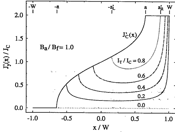
FIG. 11. Calculated added current profiles J'_y(x) in the case of nonmonotonic application of a field, followed by the application of a transport current in thin-film geometry. The solid curve shows the spatial dependence of the available critical-current density after the initial application of the field B_a = B_f . The rest of the curves show the added current profiles as I_T is increased from 0 to 0.8I_c . At I_T = I_c the added current distribution equals J'_c(x) . The delimiters at the top show the position of the various parameters for the case of B_a = B_f and I_T = 0.8I_c .
