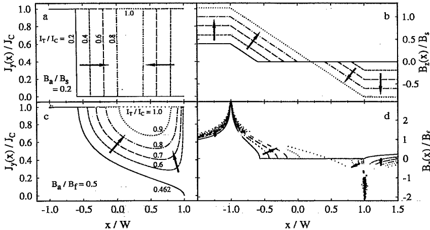
FIG. 8. Calculated critical-state behavior in monotonically increasing field and current in the high-current-low-field regime. The current-density and magnetic-flux-density profiles for slabs are shown in (a) and (b), and the corresponding profiles for films are shown in (c) and (d). The solid curves show the profiles corresponding to the matching conditions of field and current such that no current flows at the right edge of the sample. Arrows indicate the progression of the profiles as I_T is increased which results in generating currents which flow in the same direction on both sides of the sample.
