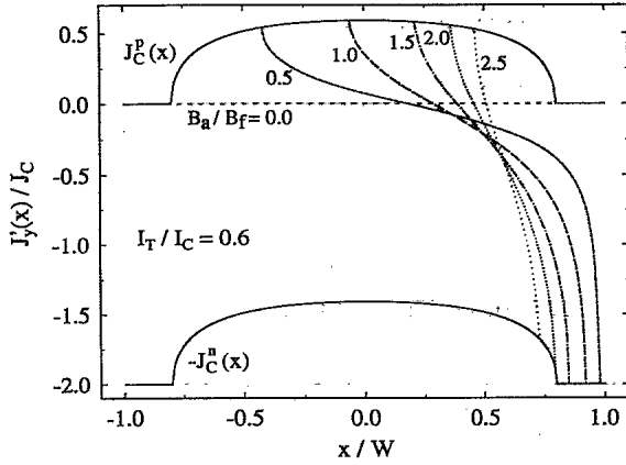
FIG. 14. Calculated added current profiles J'_y(x) in the case of nonmonotonic application of transport current followed by the application of a magnetic field in thin-film geometry. The solid curves show the available critical-current-density profiles for generating currents flowing in the positive y direction, J_c^p(x) , and in the negative direction, J_c^n(x) , following the initial application of I_T = 0.6I_c . The remaining curves show the added current profiles as B_a is increased from 0 to 2.5B_f .
