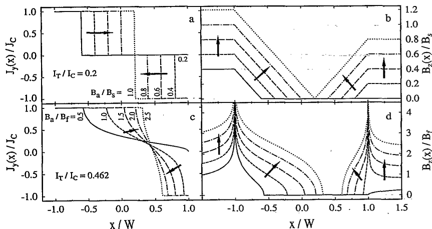
FIG. 9. Calculated critical-state behavior in monotonically increasing field and current in the low-current-high-field regime. The current-density and magnetic-flux-density profiles for slabs are shown in (a) and (b), and the corresponding profiles for films are shown in (c) and (d). The solid curves show the profiles at the same matching conditions as in Fig. 8. Arrows indicate the progression of the profiles as B_a is increased, which results in generating currents that flow in different directions on opposite sides of the sample.
