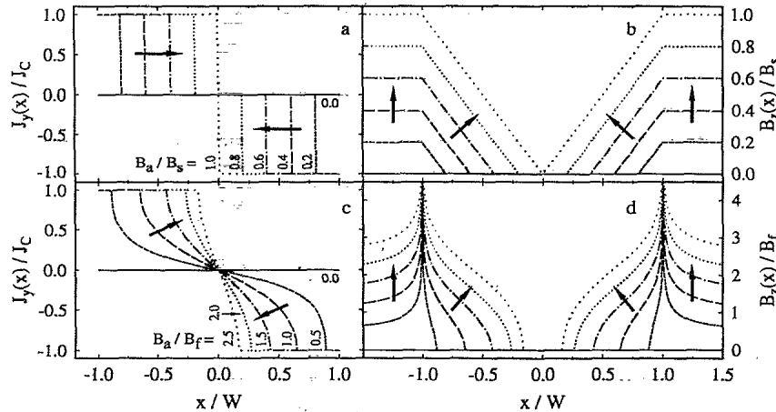
FIG. 2. Calculated critical-state behavior as the applied field B_a is increased for a sample initially in the virgin state. The current-density and magnetic-flux-density profiles for a slab are shown in (a) and (b), and the corresponding profiles for a film are shown in (c) and (d). Arrows indicate the progression of the profiles as B_a increases.
