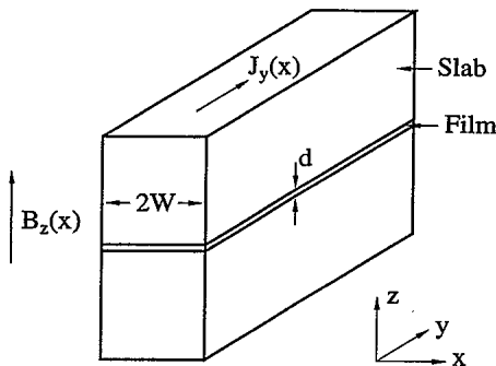
FIG. 1. Schematic diagram of slab and film geometries considered in this paper. The origin of our coordinate system is at the center of the slab or film.
