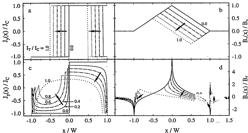
FIG. 7. Calculated critical-state behavior for a sample, initially in a fully penetrated remanent state, to which an applied transport current is raised to an intermediate value I_T and then reduced to zero. The current-density and magnetic-flux-density profiles for slabs are shown in (a) and (b), and the corresponding profiles for films are shown in (c) and (d). The solid curves show the profiles for the remanent state, and arrows indicate the progression of the profiles for increasing intermediate values of I_T . Since the final transport current is zero, the integral of J_y(x) is zero in each case.
