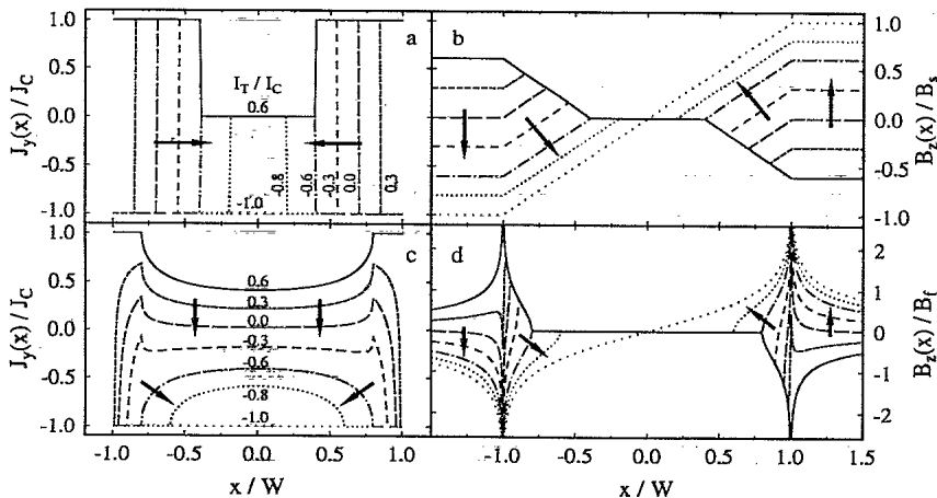
FIG. 6. Calculated critical-state behavior as the transport current I_T is decreased for a sample initially carrying current I_T = 0.6I_c in a partially penetrated state shown in Fig. 3. The current-density and magnetic-flux-density profiles for slabs are shown in (a) and (b), and the corresponding profiles for films are shown in (c) and (d). The solid curves show the initial I_T = 0.6I_c profiles, and arrows indicate the progression of the subsequent profiles as I_T decreases. The entire cross section finally attains the critical state when I_T = -I_c .
