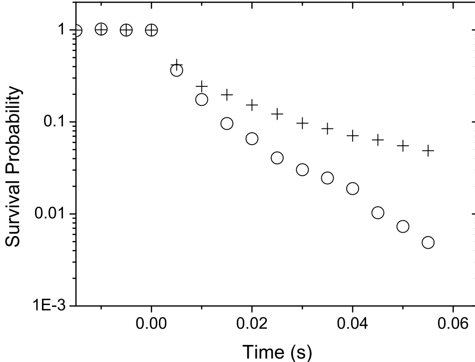
Fig. 4. Experimental results for the decay of cold atoms from a tilted-stadium shaped atom-optics billiard, with two different values for the softness parameter: w_0 = 14.5\mu\text{m} ( \circ ), and w_0 = 24\mu\text{m} ( + ). The hole is located inside the big semicircle. The smoothing of the potential wall causes a growth in stability, and a slowing down in the decay curve.
