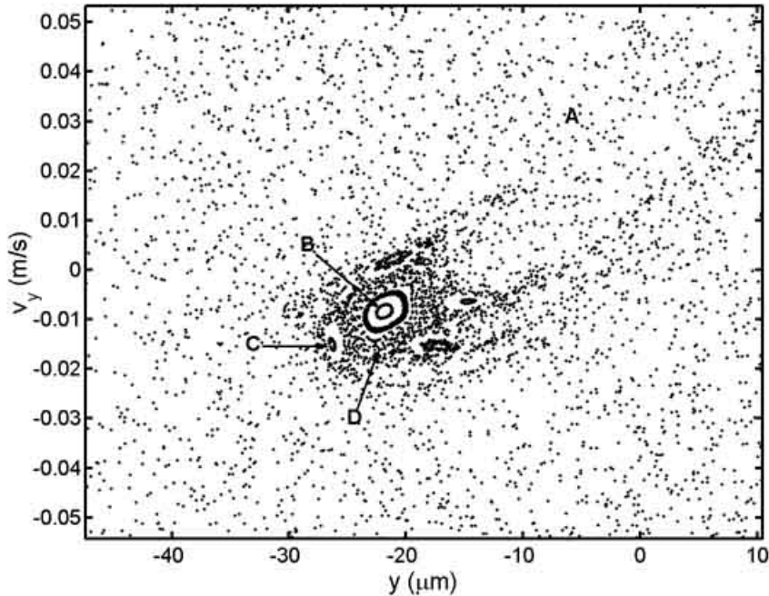
Fig. 6. Poincaré surface of section calculated for monoenergetic atoms confined in the soft dispersing billiard described in the text with \zeta = 40 \mu\text{m} and w_0 = 24 \mu\text{m} . The Figure shows \sim 17\% of the total phase space area. Phase space area corresponding to chaotic trajectories are marked "A", those of period 2 trajectories inside an island "B", areas of higher periodicity trajectories "C" and "sticky" trajectories "D".
