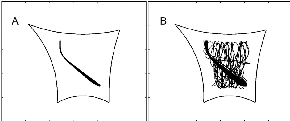
Fig. 9. Corner trajectories. (A) A periodic trajectory of period 2. (B) A "Sticky" trajectory.
