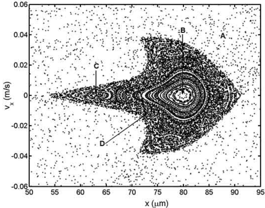
Fig. 2. Poincaré surface of section for monoenergetic atoms confined in a soft ( w_0 = 24\mu\text{m} ) tilted-stadium shaped atom-optics billiard with parameters as in Fig. 1. The Figure shows \sim 9\% of the total phase space area. A phase space area corresponding to chaotic trajectories is marked "A", one of period 2 trajectories inside an island "B", an area of higher periodicity trajectories "C" and one of "sticky" trajectories "D".
