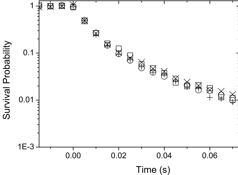
Fig. 5. Experimental results for the decay of cold atoms from a circle shaped atom-optics billiard, with different values for the softness parameter: w_0 = 14.5\mu\text{m} ( \circ ), w_0 = 18.5\mu\text{m} (+), w_0 = 21\mu\text{m} ( \square ), w_0 = 23.5\mu\text{m} ( \times ).
