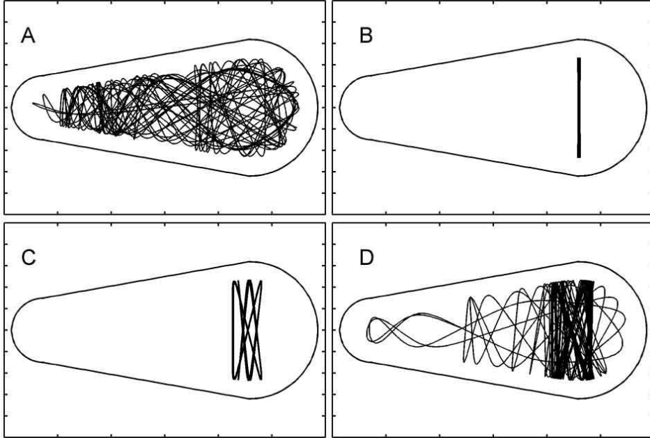
Fig. 3. Typical trajectories for atoms confined in a soft ( w_0 = 24\mu\text{m} ) tilted-stadium shaped atom-optics billiard with parameters as in Fig. 1. (A) A chaotic trajectory, corresponding to the area marked "A" in Fig. 2. (B) A periodic trajectory of period 2 and belonging to the central island, marked "B" in Fig. 2. (C) A high periodicity trajectory (Smaller islands surrounding the central one and denoted "C" in Fig. 2). (D) A "Sticky" trajectory, spending in the island's vicinity a relative long time ("D" in Fig. 2).
