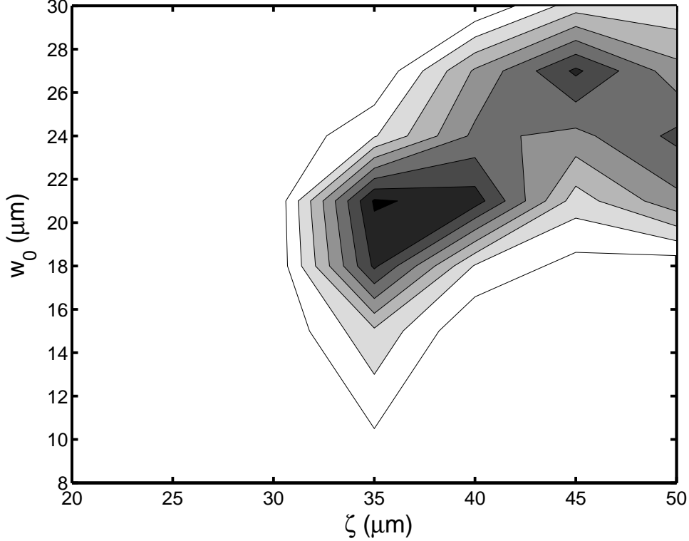
Fig. 8. Island size in the soft wall dispersing billiard, as a function of the softness parameter, w_0 , and the shape parameter, \zeta . (White - no island with an area greater than 1.6 \times 10^{-3} of the total phase space area, black - a large island, \geq 4 \times 10^{-2} of the total phase space).
