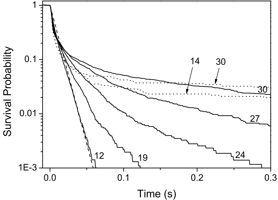
Fig. 1. Numerical simulations for the decay, through a small hole, from a tilted Bunimovich stadium (solid lines) and a circular billiard (dotted lines) with the parameters specified in the text, for several values of the softness parameter. Both billiards have the same area and hole size. The numbers adjacent to the lines indicate the value (in microns) of the softness parameter w_0 . The simulations for the stadium show a monotonic slowing down in the decay and increase in stability as the walls are made softer. For the circular billiard, there is almost no change in the decay curve as a consequence of the higher softness. The dashed line shows \exp(-t/\tau_c) , where \tau_c is the escape time calculated for the experimental parameters.
