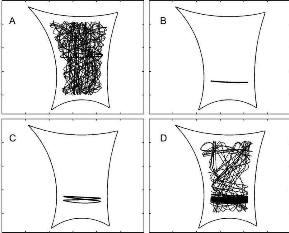
Fig. 7. Typical trajectories in a soft dispersive billiard, with the parameters as in Fig. 6, and softness parameter w_0 = 24 \mu\text{m} . (A) A chaotic trajectory. (B) A periodic trajectory of period 2. (C) A high periodicity trajectory. (D) A "Sticky" trajectory.
