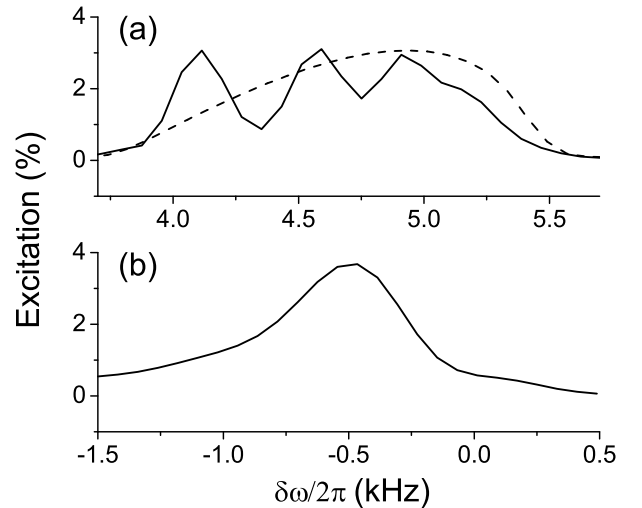
FIG. 2: Bragg and echo spectra for q = 8.06\mu m^{-1} (free particle regime). (a) Excitation spectrum of the Bragg process calculated with an exact GPE simulation (solid line) and in the LDA (dashed line). (b) Excitation spectrum of the echo scheme from a GPE simulation.
