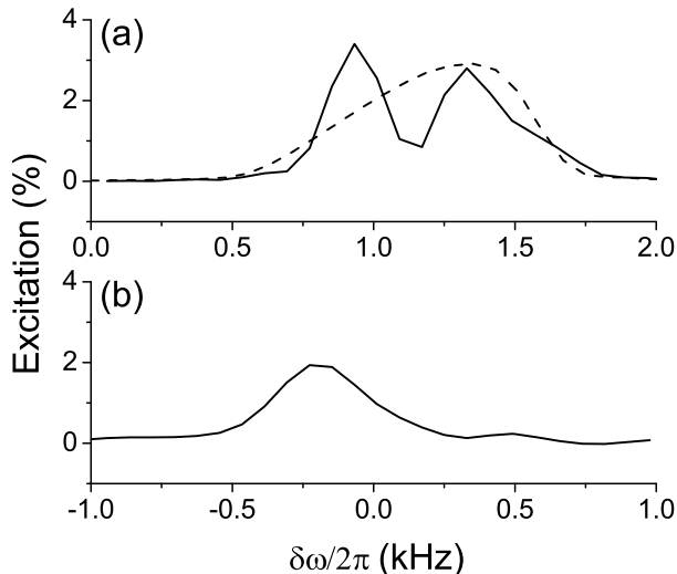
FIG. 3: Same GPE and LDA calculations as in Fig. 2, for the Bragg (a) and echo (b) spectra, only with q = 3.10\mu\text{m}^{-1} (phonon regime). We observe narrowing of the echo spectrum. In addition we note a smaller shift of the echo resonance, with respect to fig. 2b.
