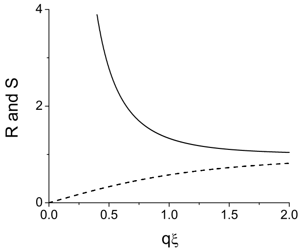
FIG. 4: The echo response R (solid line). The dashed line shows the structure factor S_q . Note the enhancement of R and the suppression of S_q for small q .
