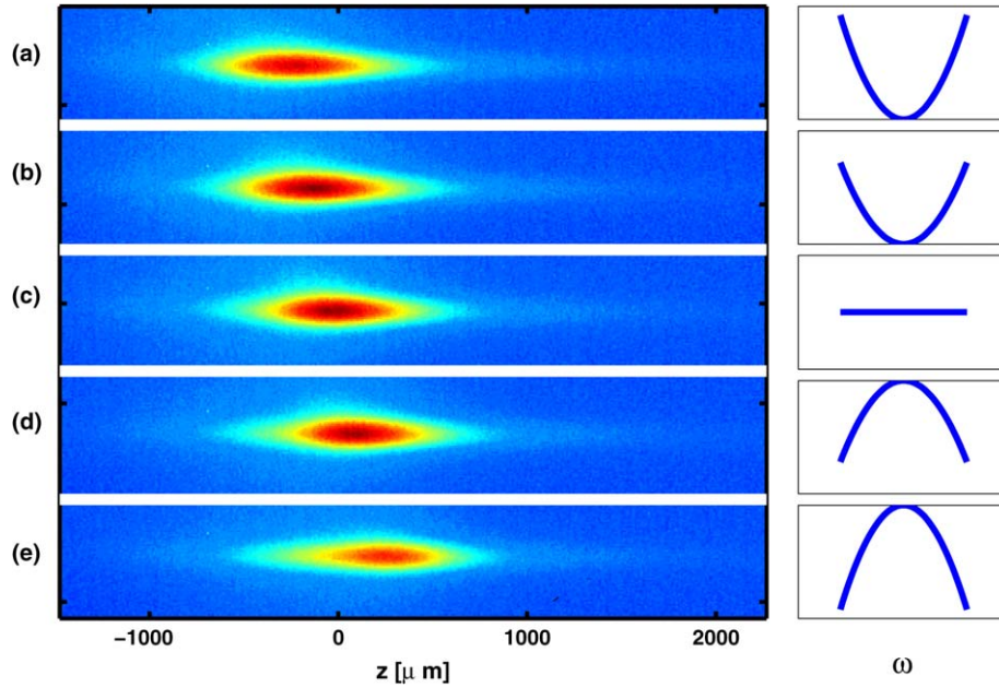
Fig. 2. The effect of GVD on the TPA spatial distribution. Shown for each image is a schematic of the spectral phase function applied on the SLM. Images correspond to GVD values ranging from (a) -10^4 [fs^2] to (e) +10^4 [fs^2] . The net effect of the applied GVD is to move the location of the temporal focus along the propagation axis.
