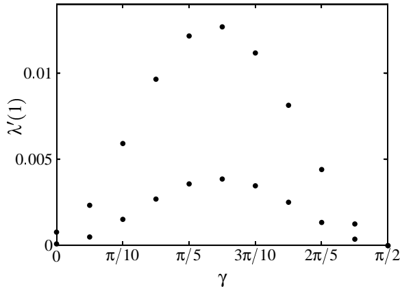
FIG. 1: Logarithmic growth rate as function of the polarization angle for two levels of the wave energy.
