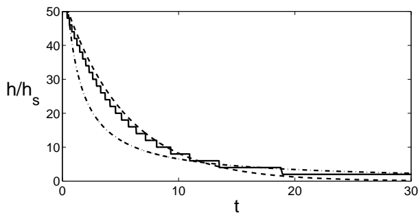
FIG. 1. Amplitude relaxation of an initially sinusoidal grating (solid line) measured in units of the height of an atomic step, h_s . The dashed and dash-dotted lines are fits to an exponential decay and an inverse linear decay, respectively. Time is in arbitrary units.
