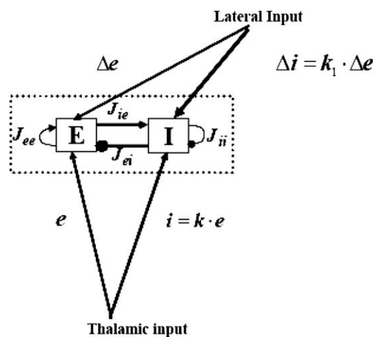
Fig. 6. A schematic representation of a cortical hyper-column (Adini et al., 1997, 2002), consisting of two interconnected sub-populations ( E -excitatory, I -inhibitory), used here to model contrast discrimination. Both E and I populations receive external input from the thalamus ( e , i ) and from within the cortex ( \Delta e , \Delta i ).
