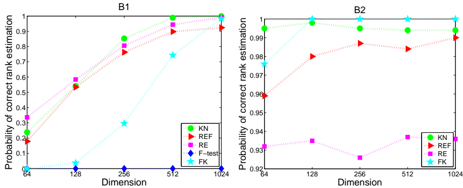
Figure 3: Empirical probability of correct rank estimation for various p and various algorithms, for settings B1(left) and B2(right): real data, K = 4 , \lambda = (200, 50, 10, 5) , c = 4 (left) or c = 1 (right). In setting B2, the performance of the F -test is at P = 0 and is not shown.
