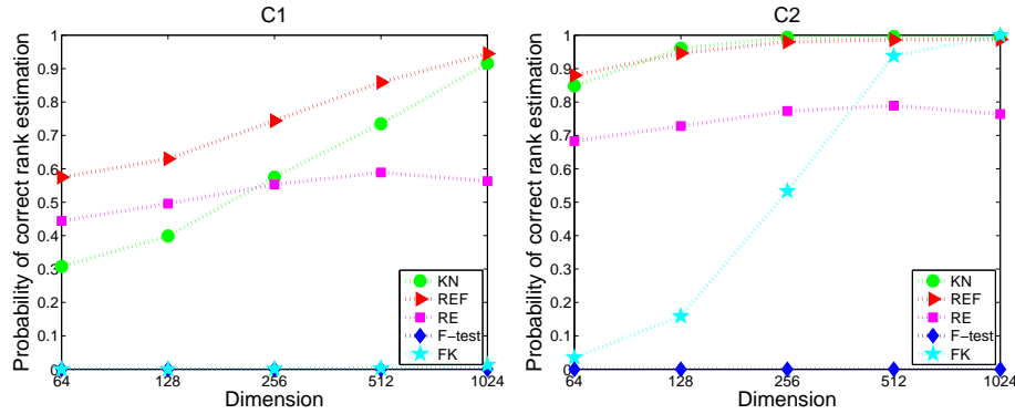
Figure 4: Empirical probability of correct rank estimation for various p and various algorithms, for settings C1(left) and C2(right): complex data, K = 2 , \lambda = (9, 2) , c = 2 (left) or c = 1 (right).
