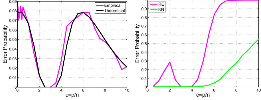
Figure 6: (Left) Empirical and theoretical probabilities of inferring an incorrect number of signals, for signal-free real-valued samples of dimension p = 1000 , for various values of the number of samples n , as a function of c = p/n . (Right) Empirical probabilities of inferring an incorrect number of signals, for real-valued samples carrying four signals with variances \lambda = (200, 100, 10, 5) , as a function of c = p/n , where p = 1000 .
