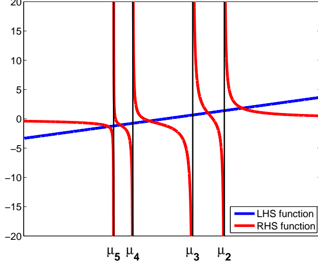
Figure 5: This figure illustrates Eq.(24). The x axis corresponds to \lambda . The blue line plots the function on the LHS of the equation, while the red line plots the function on the RHS (which diverges whenever \lambda = \mu_i ). Equality holds in Eq.(24) whenever the two curves meet. \ell_2 corresponds to the second intersection from the right, between \mu_3 and \mu_2 .
