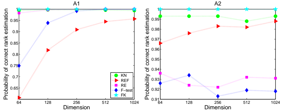
Figure 1: Empirical probability of correct rank estimation for various p and various algorithms, for settings A1(left) and A2(right): real data, K = 2 , \lambda = (200, 50) , c = 4 (left) or c = 1 (right).
