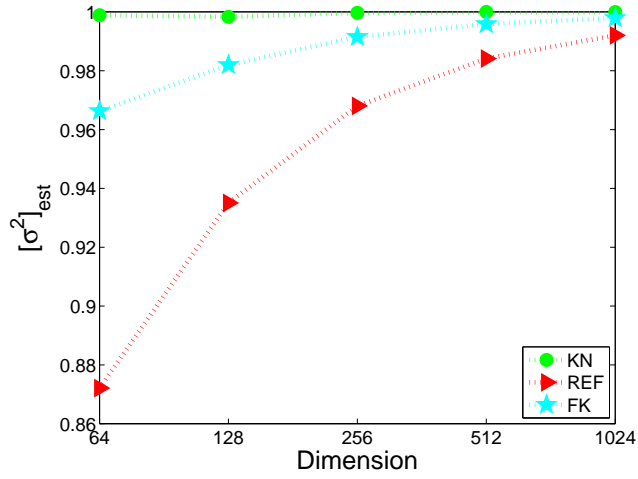
Figure 2: Empirical mean of \sigma_{est}^2 of the KN estimator, of the real error function, and of the FK algorithm, for setting A1: real data, K = 2 , \lambda = (200, 50) , c = 4 .
