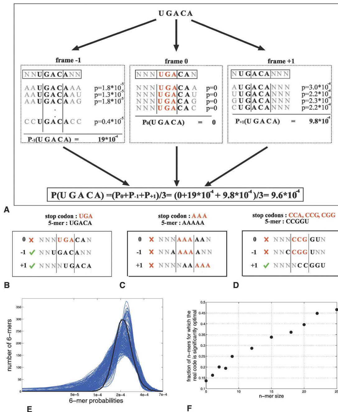
Figure 2. (A) Calculation of the probability that an n-mer sequence appears within a protein-coding region in the real genetic code. The 5-mer sequence S = UGACA can appear in one of the three reading frames. For each reading frame, the probabilities of all three codon combinations that contain S are summed up. Codon combinations with an in-frame stop (such as UGA ) do not contribute to the n-mer probability since they cannot appear in a coding region. Vertical lines separate consecutive codons, stop codons are in red, P_0 , P_{-1} , P_{+1} denote the probabilities of encountering S in the 0/-1/+1 frame. (B,C,D) Three examples of “difficult” n-mers in the real code and in alternative codes. (B) The 5-mer UGACA , which includes the stop codon UGA , can appear in a protein-coding sequence with the real genetic code in only two of the three possible reading frames (+1 and -1 frames). (C) In the alternative code shown in Figure 3D, whose stop codon AAA overlaps with itself, the 5-mer AAAAA cannot appear in a protein-coding sequence in any of the three reading frames. (D) In an alternative code with the overlapping stop codons CCG and CGG , the 5-mer CCGGU can only appear in one reading frame. The 5-mers are in bold text, stop codons are in red, N denotes any DNA letter, green \checkmark denotes a frame in which the n-mer can appear, red \times denotes a frame in which the n-mer cannot appear. (E) Distribution of the probabilities of all 6-mers in the real code (bold black line) and in the alternative codes (light blue lines). The x-axis is the probability of obtaining 6-mers within protein-coding sequences; the y-axis is the number of 6-mers with this probability. In the real code there are significantly less “difficult” 6-mers (with low probabilities), relative to the alternative codes. (F) The fraction of n-mers that have a higher probability in the real code than in alternative codes increases with n-mer size. The y-axis shows the fraction of n-mers for which the average probability of appearing in the real genetic code is significantly higher than in the alternative codes.
