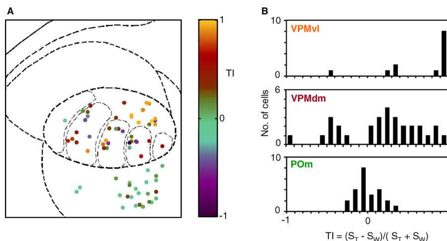
Figure 3. Distributions of Normalized Touch Responses in the Thalamus
