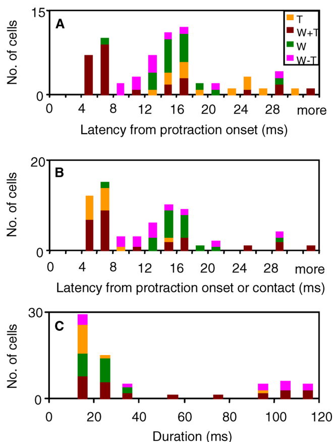
Figure 4. Distributions of Thalamic Latencies and Durations According to Response Type
