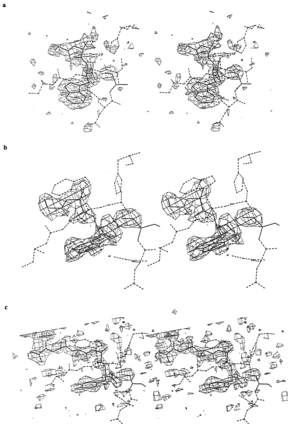
FIGURE 4: "Omit" difference electron density maps drawn in stereo, showing the bound oligopeptide (solid line) in the active site of the enzyme (dashed line). The maps were calculated with amplitudes of (F_o - F_c) and phases from \gamma -Cht after seven additional cycles of refinement omitting the putative oligopeptide and the side chain of Ser195. Contours drawn at 2\sigma . (a) Omit map for Nat-1 showing the putative tripeptide Gly-Ala-Trp and the neighboring residues. (b) Omit map for Nat-2 showing the putative tripeptide Gly-Ala-Trp and the neighboring residues as above. (c) Omit map for Nat-3 showing the putative pentapeptide Ala-Ala-Ala-Ala-Tyr and the neighboring residues as above.
