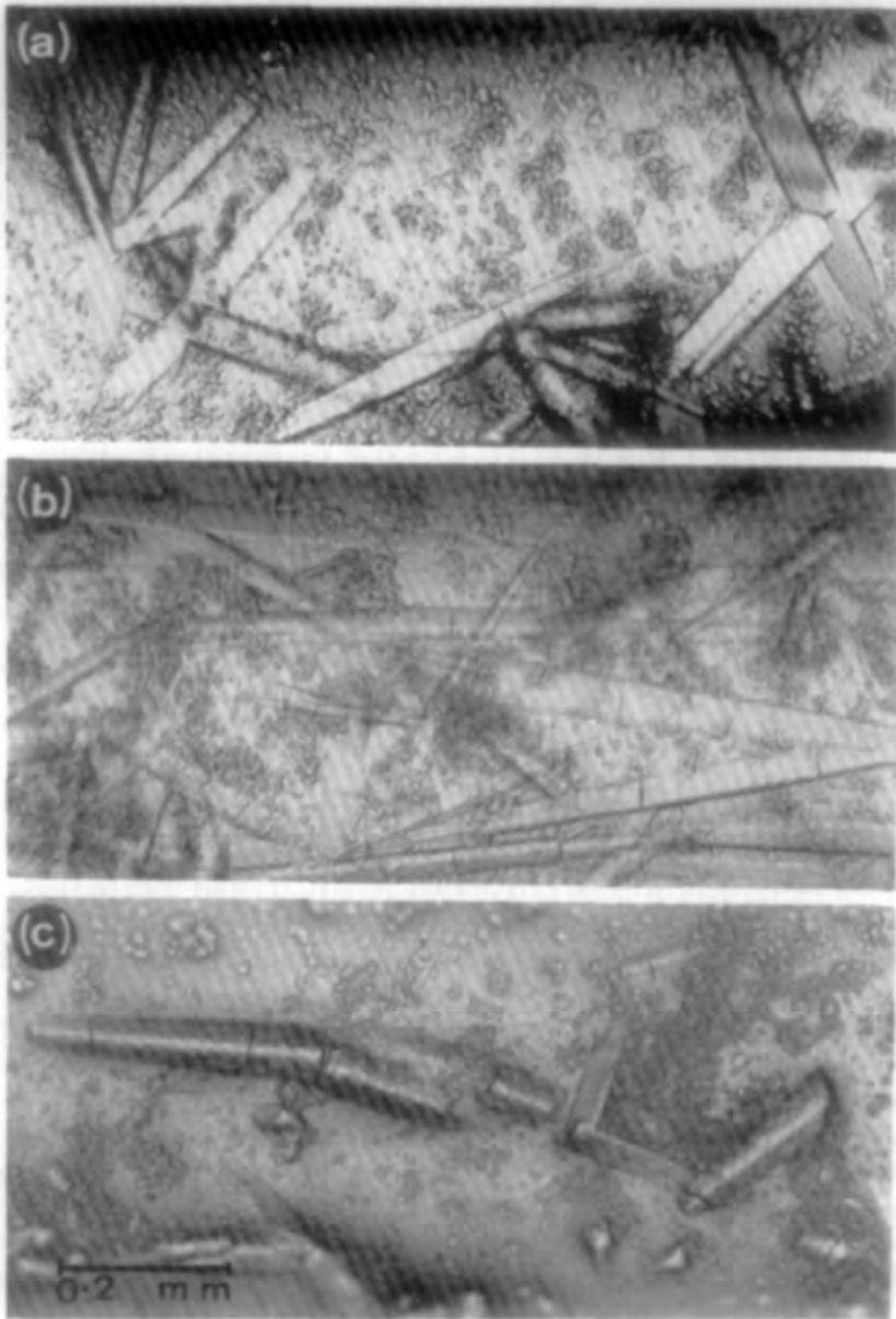
FIG. 2. Development of cracks with crystal growth. Crystals have been obtained as described by Yonath et al. (1982a) from 30% methanol at pH 8.4, and are shown after; (a) 25 and (b) 40 days of growth. (c) Cracked crystals which have been grown from a mixture of 17% (v/v) ethylene glycol and 17% methanol (pH 8.4).
