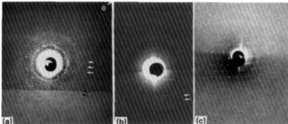
FIG. 3. Still diffraction patterns, obtained with synchrotron radiation at X11/DORIS under parasitic conditions at about 5 GeV and 22 to 28 mA, with 0.12 mm aperture, at 12 to 15°C for about 1 h. From:
