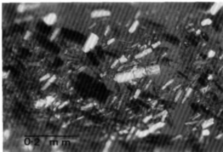
FIG. 1. Crystals, grown from 30% (v/v) methanol at pH 8.7, using a modified version of the crystallization method described by Yonath et al. (1982a); i.e. addition of 1% alcohol to the crystallizing solution and seen under polarized light.
