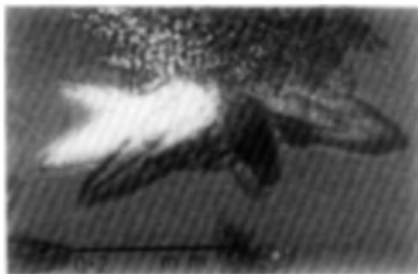
Fig. 4. Crystals grown in hanging drops as described by Yonath et al. (1982 a ) from 10% ethylene glycol at pH 7.8 and seen under polarized light.
