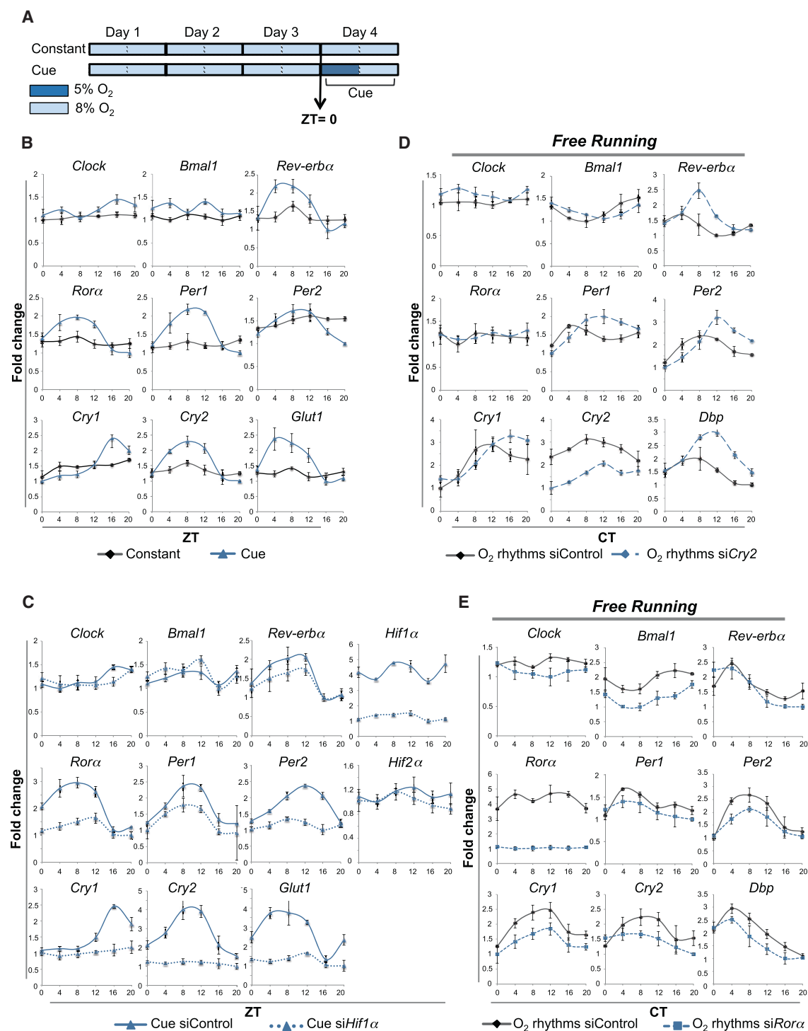
Figure 3. Specific Clock Genes Respond to Changes in Oxygen Levels in a HIF1 \alpha -Dependent Manner
