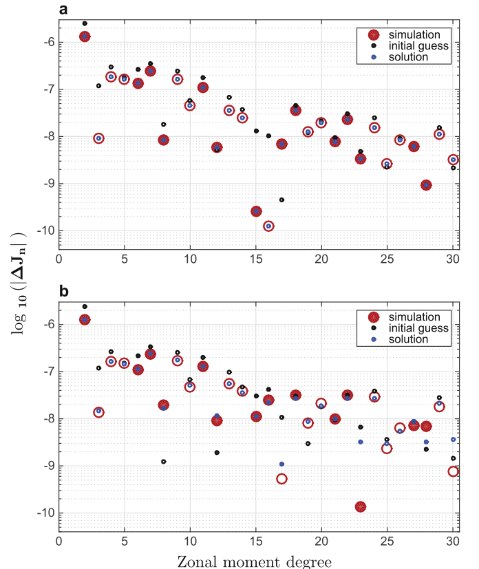
Figure 3. Jupiter gravitational moments for (a) a case with no errors in the simulated moments, and (b) a case with random errors. Shown are the simulation (red), initial guess (black), and solution (blue). Filled (open) circles denote positive (negative) values.
