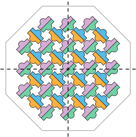
Pure Host
