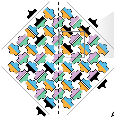
Mixed Crystal
