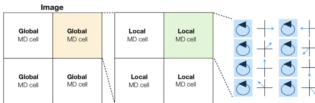
Fig. 5. Tiled architecture of the direction sensitive MD cells. Each oscillator has its own preferred direction. Every 8 oscillators constitute a local motion detector (MD) cell. Each 4 neighboring local MD cells comprise a global MD cell, which are evenly distributed over an image.
