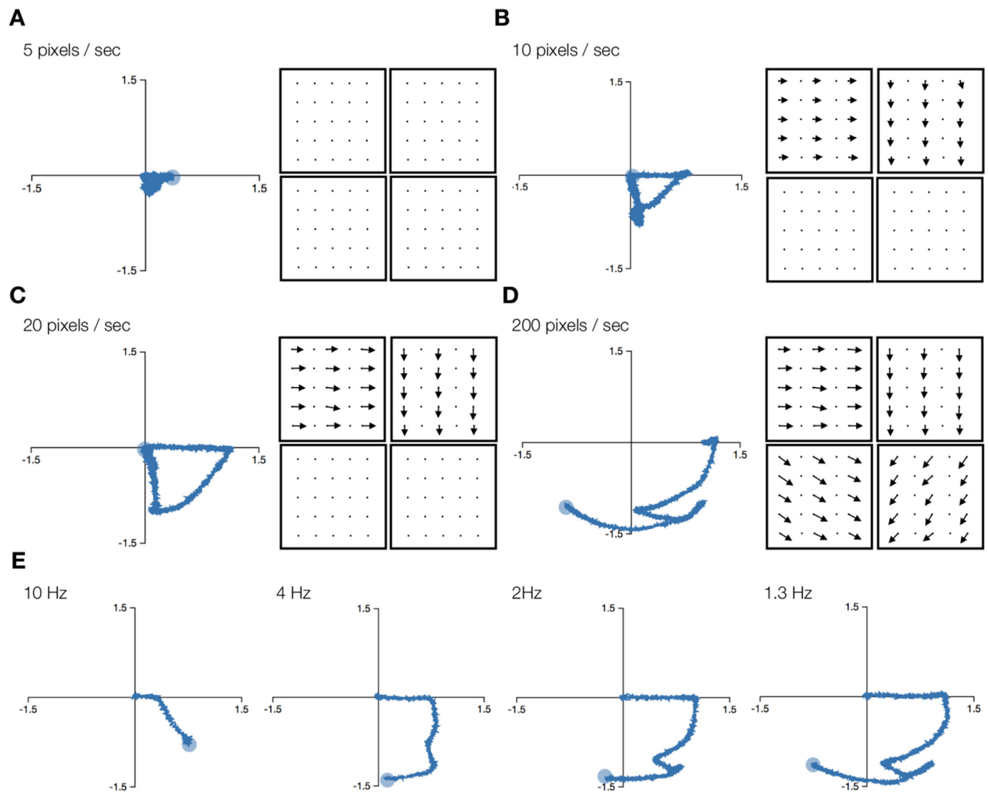
Fig. 7. Global MD cell response to drifting grating. 5 \times 5 global MD cells were evenly distributed across the image. Same visual stimuli were used here as in Fig. 4, only in varying velocities and frequencies. (A–D) pattern drifting times are 5, 10, 20, and 200 pixels/s respectively, gained by moving 2.5%, 5%, 10%, 100% of the gratings image width in 1 s intervals. In each panel, the state space of the middle global MD cell is shown on the left, and an arrow field, where each dot/arrow signifies the detected motion direction of one localized global MD cell. (E) Applying the same stimuli in different pattern switching frequencies ranging from 10 to 1.3 Hz, gained by moving 10%, 25%, 50%, 75% of the grating image width in 0.1, 0.25, 0.5 and 0.75 s, while preserving drifting velocity of 200 pixels/s.
