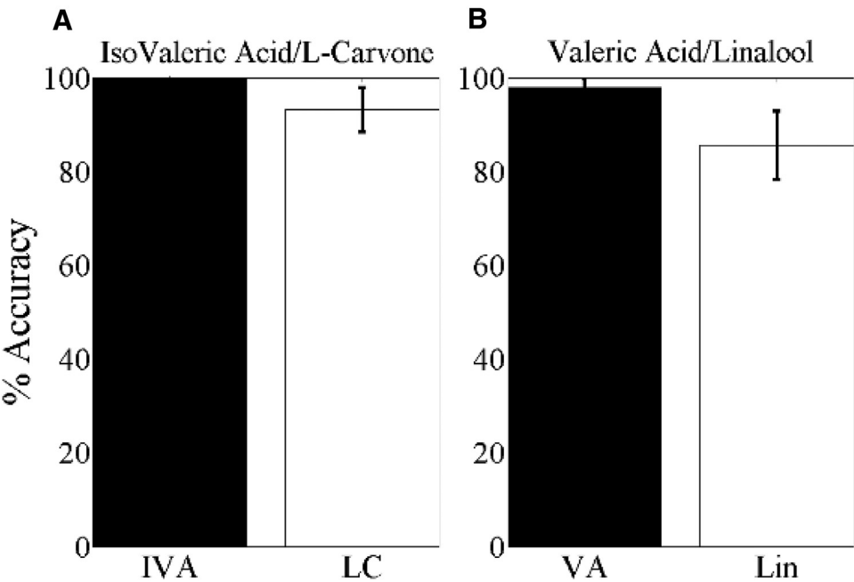
FIG. 6. Odorant classification from EOGs within subjects. Percent accuracy in EOG classification by the stimulating odorant at 100% > for either of the pairs. A: iso-valeric acid (50% olfactometer dilution) vs. L-carvone (50% olfactometer dilution) or B: valeric acid (50% olfactometer dilution) vs. linalool (50% olfactometer dilution) . Classification was carried out by the minimal least squared distance between the tested EOG curve and the remaining EOGs within a subject's dataset (Eq. 6).
