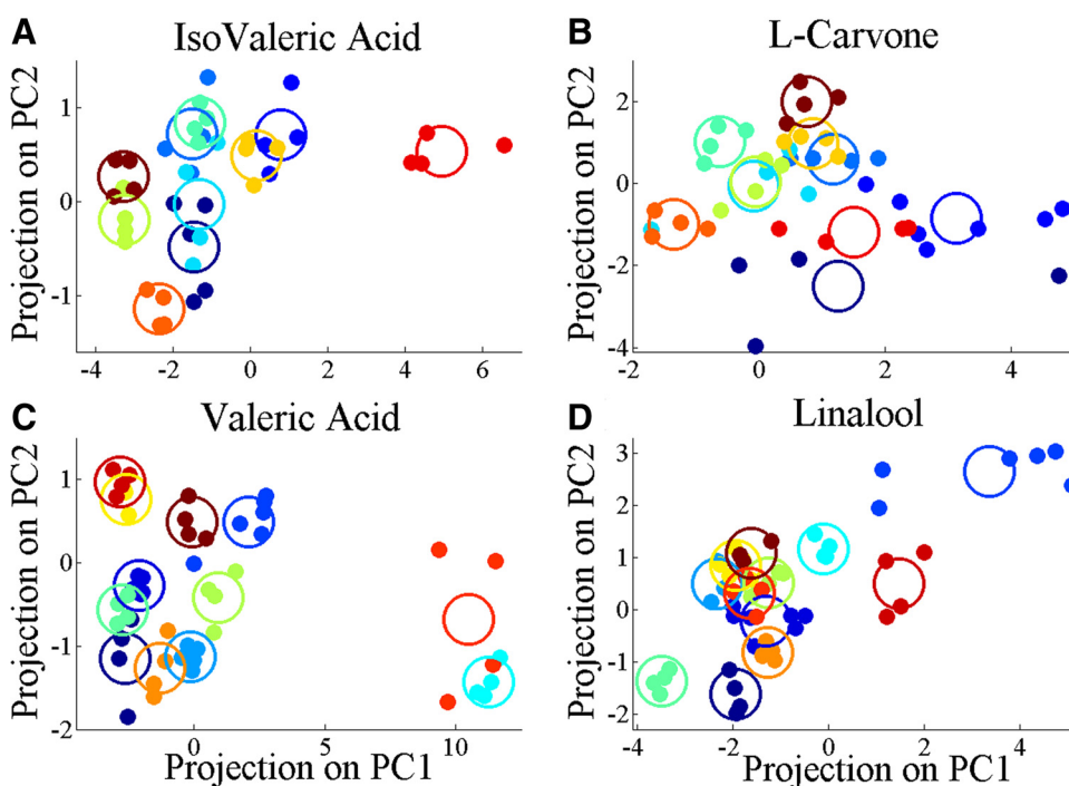
FIG. 2. PCA of EOGs. Principal component analysis computed on the raw EOG signals of the two odorant pairs between t = 0.5 s and t = 2.5 s: A: iso-valeric acid (50% olfactometer dilution); B: l-carvone (50% olfactometer dilution) both with n = 10 ; C: valeric acid (50% olfactometer dilution); and D: linalool (50% olfactometer dilution) both with n = 12 . Plotted are the projections of the raw EOG recordings on the first and second principal components (x and y axes, respectively). Each color represents a single subject with a circle around its centroid, illustrating the clustering of responses within subjects.
