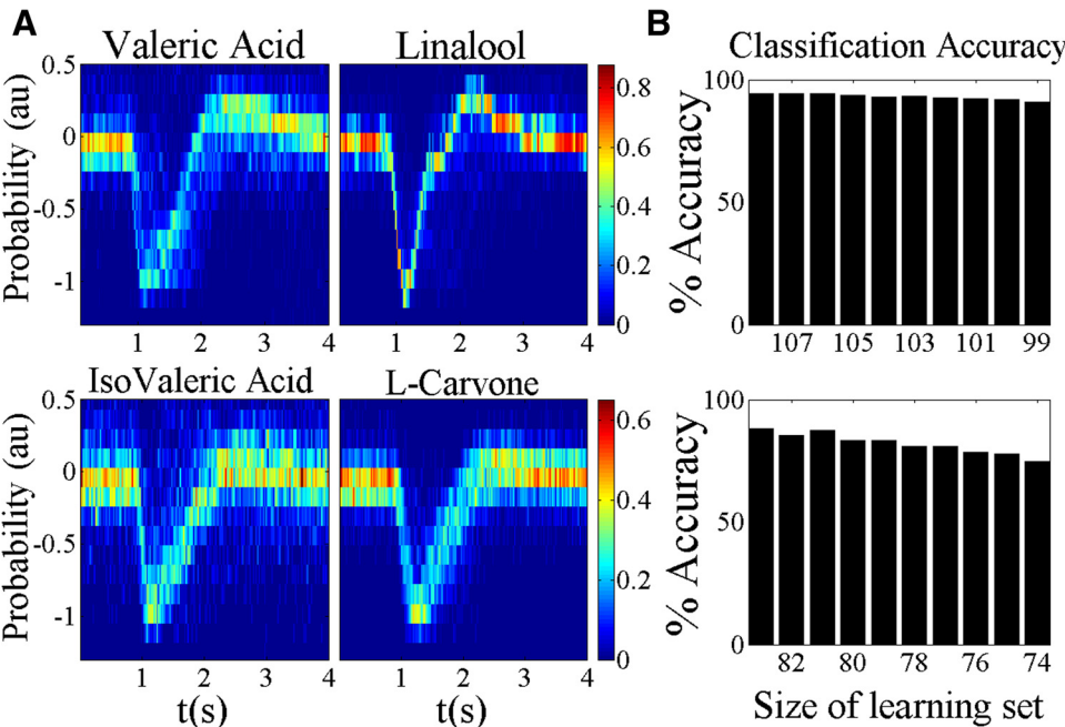
FIG. 7. Odorant classification from EOGs across subjects. A: probability distributions of the evoked EOGs calculated from the normalized learning set (Eq. 7). Y axis is the evoked response in arbitrary units (au), X axis is the time course in seconds, stimulus duration = 500 ms starting at t = 0.5s . Top: valeric acid (50% olfactometer dilution) against linalool (50% olfactometer dilution) Bottom: iso valeric acid (50% olfactometer dilution) against L-carvone (50% olfactometer dilution) B: percent accuracy in odorant classification as a function of the size of the learning set. The tested odorants correspond to the probability plots of their learning sets shown in A.
