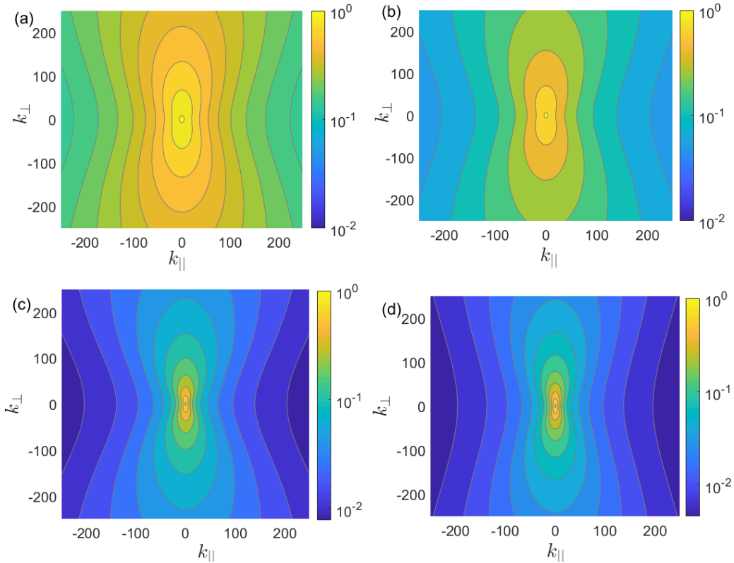
Figure 2. The K41-compensated 2D energy spectra k^{8/3}\mathcal{E}(\mathbf{k}) . Panels (a), (b): the spectra are calculated for k_{\times} = 100 and \tilde{\Omega} = 2, 5 respectively. Panels (c), (d): the spectra are calculated for k_{\times} = 20 and the same values of \tilde{\Omega} . Note logarithmic scale of the color-bars. The contour levels are spaced by 0.1 in (a) and (b) and by 0.2 in (c) and (d).
