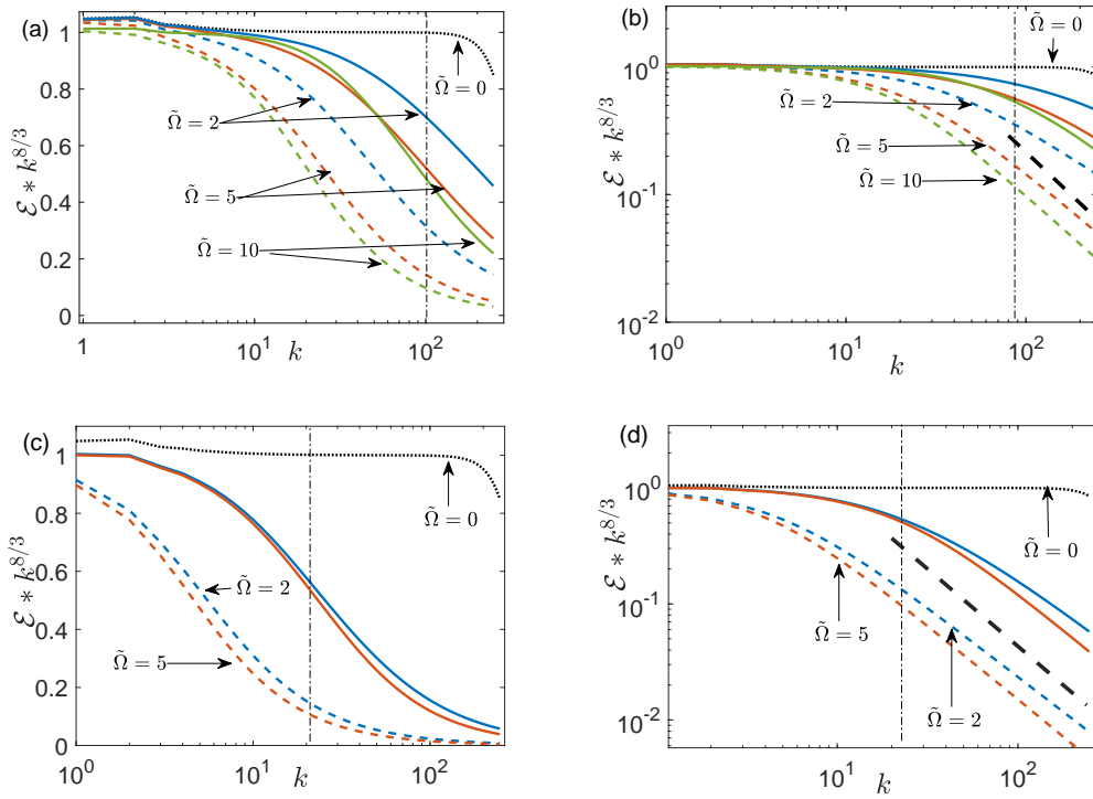
Figure 3. Numerical solution of Eq. (1.13). The K41-compensated spectra along k_{\parallel}^{8/3}\mathcal{E}(k_{\parallel}, 0) and normal to the counterflow direction k_{\perp}^{8/3}\mathcal{E}(0, k_{\perp}) . The values of \tilde{\Omega} are indicated in the figure. In (a) and (b) k_{\times} = 100 , in (c) and (d) k_{\times} = 20 . The reference case \tilde{\Omega} = 0 (no mutual friction) is plotted in all panels by a black dotted line. Vertical dot-dashed lines denote the position of the crossover wavenumber k_{\times} . Black thick dashed lines in (b) and (d) denote \mathcal{E} \propto k^{-4} and serve to guide the eye only. Vertical dot-dashed lines indicate the position of k_{\times} . Note the log-linear scales in (a) and (b) and the log-log scales in (c) and (d).
