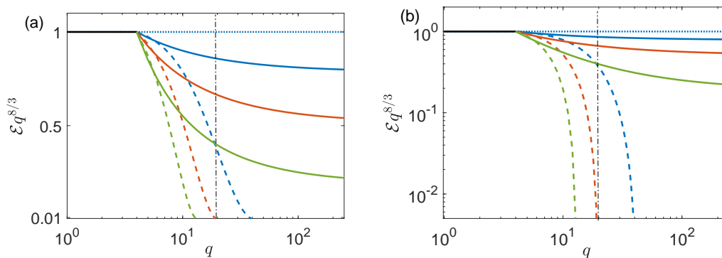
Figure 1. The K41-compensated spectra in direction of the counterflow Eq.(2.4), q_{\parallel}^{8/3}\mathcal{E}(k_{\parallel}, 0) = \Psi_{\parallel}^2(q_{\parallel}) (dashed lines) and in the orthogonal direction, Eq.(2.6b), q_{\perp}^{8/3}\mathcal{E}(0, k_{\perp}) = \Psi_{\perp}^2(q_{\perp}) (solid lines). The parameters of the spectra q_{\times} = 20 , \omega_{\text{dis}} = 0.7\tilde{\Omega} and q_* = 4 . Three sets of lines from top to bottom correspond to \tilde{\Omega} = 2 (blue lines), \tilde{\Omega} = 5 (red lines) and \tilde{\Omega} = 10 (green lines). Note the log-linear scales in (a) and the log-log scales in (b). Vertical black dot-dashed line denotes the q_{\times} = 20 .
