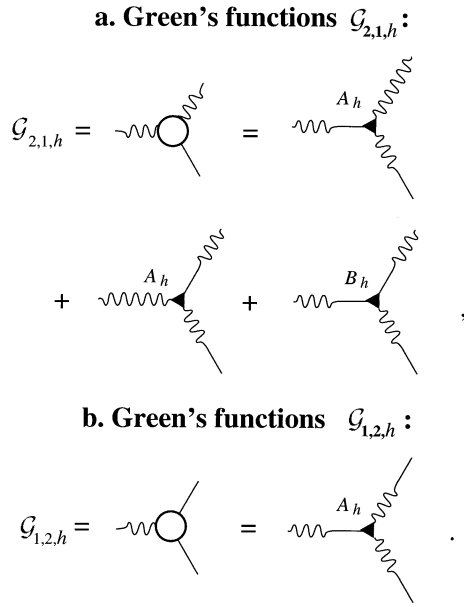
Fig. 3. This figure completes the definition of the three vertices in terms of the 3rd order correlation and Green's functions.
