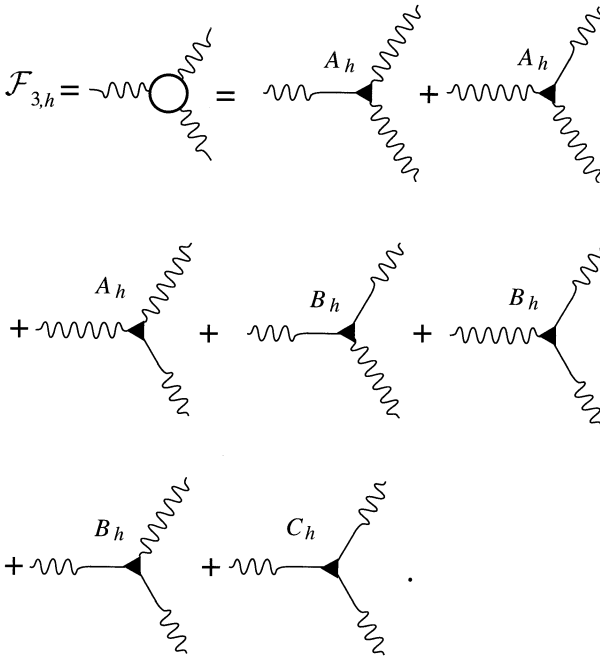
Fig. 2. The representation of the 3rd order correlation function on an “h-slice” in terms of 2-point quantities and three vertices. Note that this is not a perturbative expansion, but a definition of the vertices on an “h-slice”. The definition of the vertices is completed in Fig. 3.
