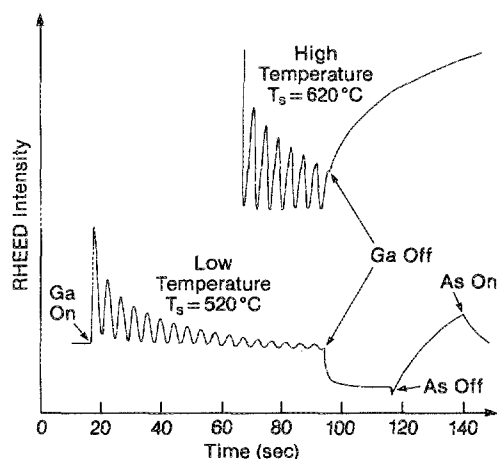
FIG. 2. A typical time evolution of RHEED specular beam intensity taken from (001)\text{-}2\times 4 reconstruction surface, during the growth and recovery of GaAs at 520^\circ\text{C} (bottom) and at 620^\circ\text{C} (top).
