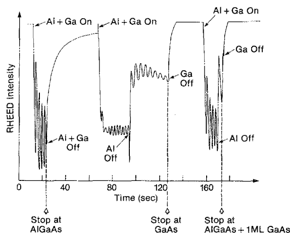
FIG. 1. A typical time evolution of RHEED specular beam intensity taken from (001)-2×4 reconstructed surface, during the growth and recovery of: (a) an AlGaAs layer (left-hand side), (b) 10 ML of AlGaAs covered by 8 ML of GaAs (center), and (c) a few AlGaAs monolayers covered by 1 ML of GaAs (right-hand side).
