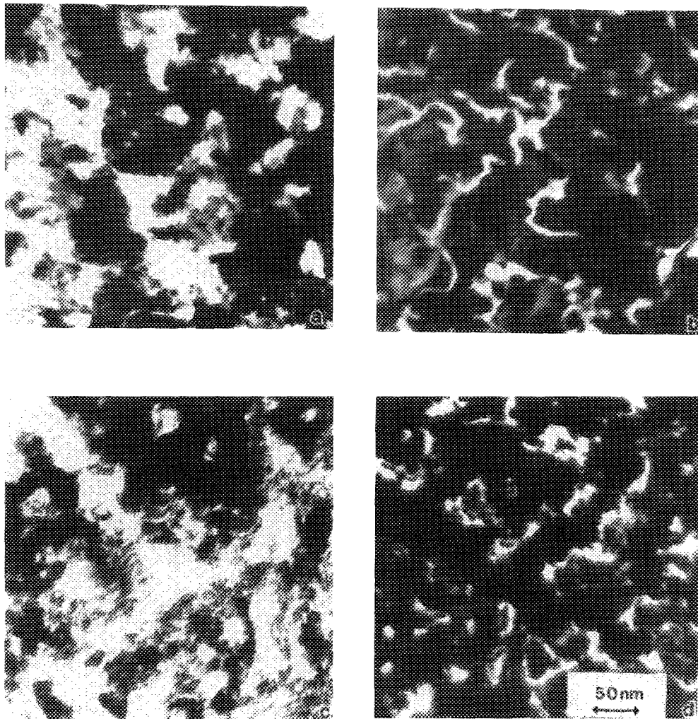
FIG. 4. (011) dark-field TEM images for (a) Mo deposited on (100)GaAs; (b) Mo deposited on ( \bar{1}\bar{1}\bar{1} )GaAs; (c) Nb deposited on (100)GaAs; (d) Nb deposited on ( \bar{1}\bar{1}\bar{1} )GaAs.
