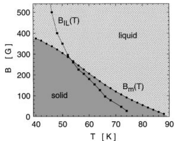
FIG. 3. The vortex-lattice melting line B_m(T) (dots) and the irreversibility line B_{IL}(T) (squares) in BSCCO crystal of prism shape. The magnetization is fully reversible above 76 K due to the absence of geometrical barrier and bulk pinning. At lower temperatures the IL is governed by surface barriers. Below 53 K the IL resides in the vortex-liquid phase, whereas at higher temperatures it crosses through the vortex-solid region. The irreversibility and melting lines in BSCCO stem from two different and unrelated mechanisms.
