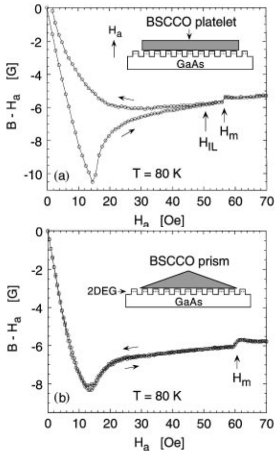
FIG. 1. Local magnetization loops B - H_a vs H_a in BSCCO crystals of platelet (a) and prism (b) shapes at T = 80 \text{ K} . The platelet crystal shows hysteretic magnetization below the irreversibility field H_{IL} . In the prism sample the geometrical barrier is eliminated and a fully reversible magnetization is obtained at temperatures above 76 \text{ K} . The melting transition H_m is observed as a sharp thermodynamic step in the local magnetization. A cross section of the experimental setup is shown schematically in the insets (not to scale). The two-dimensional electron gas (2DEG) active layer of the sensors resides about 0.1 \mu\text{m} below the surface. The BSCCO crystals are in contact with the GaAs surface and the local vertical component of the magnetic field B is measured directly. External field H_a is applied parallel to the crystalline c axis.
