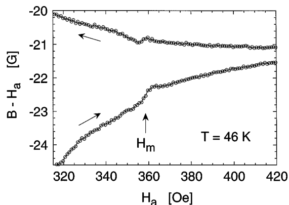
FIG. 2. Expanded view of the local magnetization loop in the prism crystal in the vicinity of the melting transition H_m at 46 K. The irreversibility field due to surface barriers is significantly higher than H_m at this temperature.
