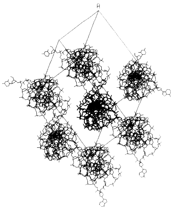
Figure 15. A packing diagram of the tridecamer structure in a view down the helix axis. The looped-out bases are seen protruding into neighboring helices: notice the looped-out base from the top helix inserting into the center helix and the looped-out base from the center helix inserting into the bottom right helix.
