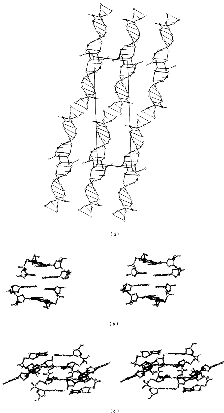
Figure 14. (a) A packing diagram of the tridecamer structure showing one layer of molecules as viewed down the crystallographic b axis. Each strand is represented by lines connecting the C_{(1)} atoms, and the base-pairs are drawn as straight lines connecting the C_{(1)} atoms on opposite strands. For the 2 extra adenine bases, a line connects the C_{(1)} (shown as filled circles) and N_{(1)} atoms. (b) Stereo drawing depicting the stacking interactions between 2 molecules (one drawn with open bonds and the other with filled bonds) around the 2-fold axis at (\frac{1}{2}, 0, \frac{1}{2}) ; (c) same as (b) around the 2-fold axis at the origin. The terminal base-pair is frayed in each molecule and the stacking is between the 2nd base-pair, C2-G25, in each molecule.
