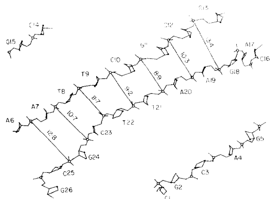
Figure 16. Cylindrical projection of the native DNA tridecamer structure showing phosphorus-phosphorus distances across the minor groove to be narrower in the center of the structure, in the vicinity of the AT-rich region, and more open at the 2 ends of the duplex (GC-rich region).
