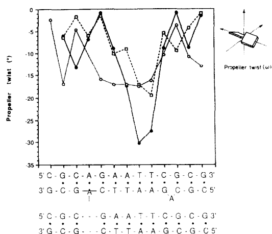
Figure 17. Observed propeller twist angles for the native tridecamer (filled circles), the proflavin-soaked tridecamer (open squares) and the Dickerson–Drew native dodecamer (open circles). All structures exhibit a large propeller twist in the AATT region. Sequences are given for the tridecamers (top) and for the dodecamer (bottom). Note that the 2 strands of the dodecamer were swapped for comparison with the tridecamer structures for reasons explained in the discussion about helix bending (see the text).
