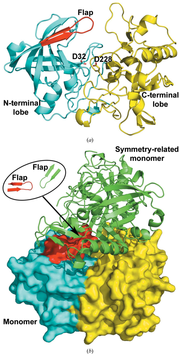
Figure 1 ( a ) Ribbon representation of the three-dimensional structure of apo BACE1. The N- and C-terminal lobes are coloured cyan and yellow, respectively. The Asp-dyad residues, Asp32 and Asp228, are displayed as sticks. Residues 67–78 (including the flap) are coloured red and the flap is shown in its ‘open’ conformation. ( b ) Ribbon and molecular-surface representations of the three-dimensional structure of the BACE1 ‘dimer’ generated based on PDB entry 1w50. The monomer is displayed in space-filling format. The symmetry-related monomer is displayed in ribbon format. A close-up of two the two flaps in the ‘dimer’ is displayed in the top left corner.
