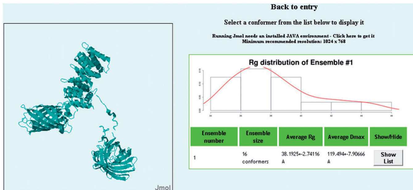
Figure 3. Jmol applet and list of conformers. Entries in pE-DB may have multiple ensembles, which may fit equally well the underlying experimental data. By navigating to the Jmol applet screen, the user can view the R_g distribution of each ensemble, the number of conformers and the average values for the R_g and the maximal distance ( D_{max} ). By clicking on the 'Show/Hide' button, a list of the conformers appears, featuring R_g and D_{max} values and a Jmol button. Clicking on the Jmol button, every single conformer can be selected to be visualized by a fully customizable Jmol applet.
