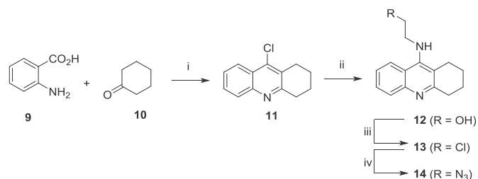
Scheme 1. Reagents and conditions. (i) POCl 3 (10.0 equiv), 0 °C, then 12 h reflux, 52%; (ii) ethanolamine (3.0 equiv), 18 h reflux, 76%; (iii) SOCl 2 (21.0 equiv), 45 min reflux, 75%; (iv) NaN 3 (4.0 equiv), DMF, 80 °C, 24 h, 61%.
