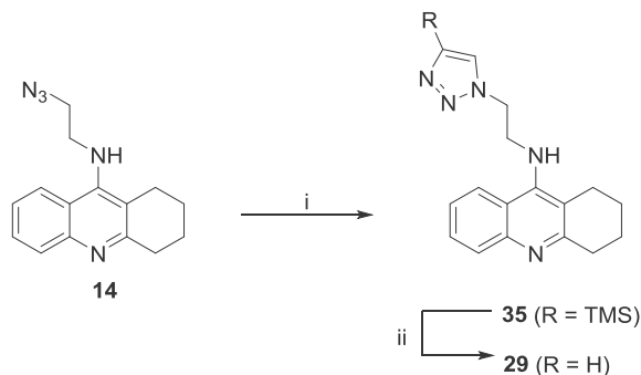
Scheme 6. Reagents and conditions. (i) trimethylsilylacetylene (1.5 equiv), CuSO 4 ·5H 2 O (0.3 equiv), sodium ascorbate (0.6 equiv), DMF, 3 h, rt, 99%; (ii) TBAF (1.0 M in THF) (2.0 equiv), THF, 3 h, reflux, 50%.
