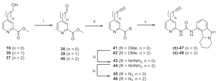
Scheme 7. Reagents and conditions. (i) IBX (3.0 equiv), EtOAc, 3 h reflux for 38 , and 12 h for 40 , 99%; (ii) Ohira–Bestmann reagent (1.5 equiv), K 2 CO 3 (2.0 equiv), MeOH, rt, 36% (for 41 ), 48% (for 42 ); (iii) hydrazine monohydrate (7.0 equiv), MeOH, 45 min, rt, 99%; (iv) NaNO 2 (2.0 equiv), 12 N aqueous HCl, 2 h, 0 °C, 64% (for 45 ), 83% (for 46 ); (v) (±)- 24 (1.0 equiv), 1,4-dioxane, 24 h, reflux, 92% (for (±)- 47 ), 40% (for (±)- 48 ).
