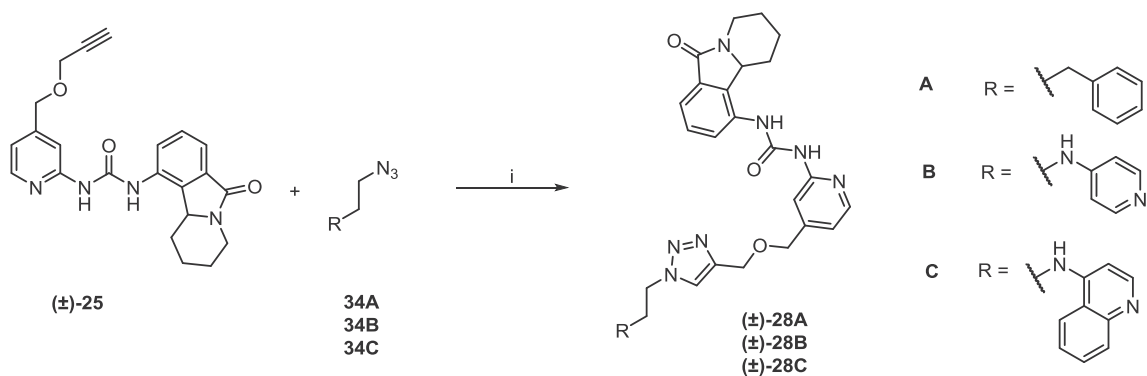
Scheme 5. Reagents and conditions. (i) 34A–C (1.0 equiv), CuSO 4 ·5H 2 O (0.3 equiv), sodium ascorbate (0.6 equiv), DMF, 48 h, rt, 99% (for (±)- 28A ), 41% (for (±)- 28B ), 47% (for (±)- 28C ).
