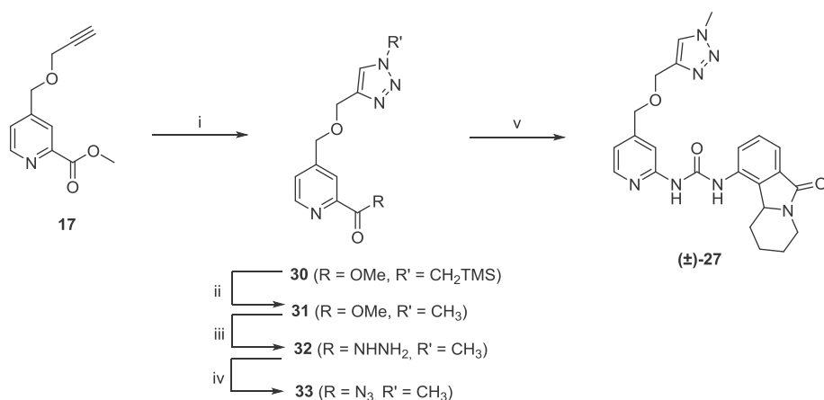
Scheme 4. Reagents and conditions. (i) trimethylsilylmethyl azide (1.1 equiv), CuSO 4 ·5H 2 O (0.3 equiv), sodium ascorbate (0.6 equiv), DMF, 24 h, rt, 74%; (ii) TBAF (1.0 M in THF) (2.0 equiv), THF, 0 °C, then 24 h rt, 76%; (iii) hydrazine monohydrate (7.0 equiv), MeOH, 45 min, rt, 99%; (iv) NaNO 2 (2.0 equiv), 12 N aqueous HCl, 2 h, 0 °C, 25%; (v) (±)- 24 (1.0 equiv), 1,4-dioxane, 24 h, reflux, 25%.
