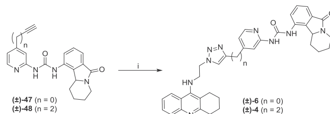
Scheme 8. Reagents and conditions. (i) 14 (1.0 equiv), CuSO 4 ·5H 2 O (0.3 equiv), sodium ascorbate (0.6 equiv), DMF, 48 h, rt, 18% for (±)- 6 , and 19% for (±)- 4 .
