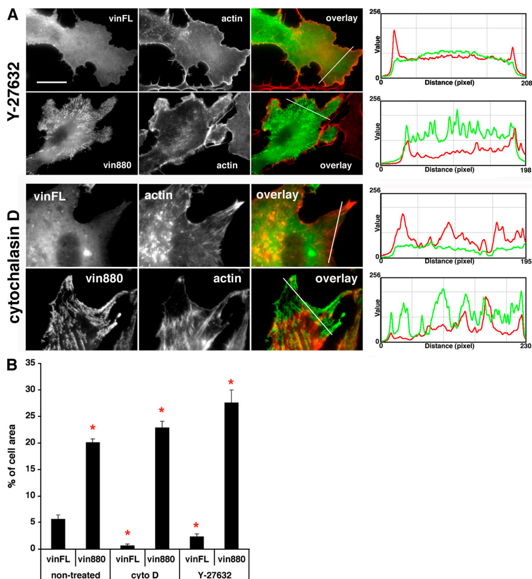
Figure 8. Vinc80 stabilizes adhesion sites in cells despite the inhibition of actomyosin function or disruption of actin filaments. (A, top) NIH3T3 cells expressing YFP-vinFL or -vin880 treated with 100 \mu M Y-27632 for 60 min. Although only small dotlike adhesions (focal complexes) can be seen at the cell periphery in vinFL-expressing cells, a large number of adhesion sites are still apparent in cells expressing vin880, despite the absence of stress fibers. (bottom) Cells treated with 1 \mu M cytochalasin D for 30 min. Although essentially no adhesions can be seen in YFP-vinFL-expressing cells, many adhesion sites are still visible in YFP-vin880-expressing cells. Fluorescence intensity profiles on the right are from the area of the line drawn in image overlays. Note that there is little if any correlation of high vinFL or vin880 intensity peaks with those of actin. Bar, 12 \mu m. (B) Quantification of FA area. FA area was calculated as a percentage of the total cell area. Note the significant loss in FA area in vinFL-expressing cells when treated with cytochalasin D (cyto D) or Y-27632. No loss of adhesion area was found in vin880 cells treated with actin-perturbing reagents. Asterisks indicate significant differences of values compared with nontreated vinFL ( P < 0.001 , HSD test). The apparent slight increase of vin880 FA area in vin880-expressing cells treated with cytochalasin D or Y-27632 compared to nontreated cells was caused by a decrease in total cell area (in the case of cytochalasin D) or increased de novo formation of adhesions at the cell periphery (in the case of Y-27632).
