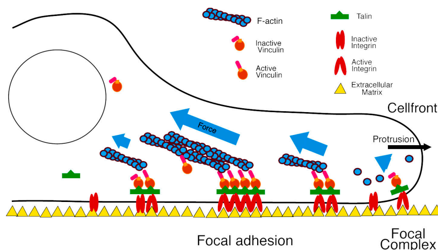
Figure 9 . Model of vinculin action in cells. See text in Discussion.
