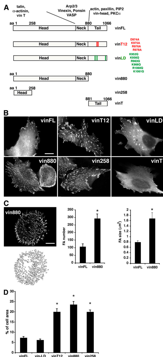
Figure 1. Effect of wild-type and mutant forms of vinculin on FA growth. (A) Vinculin constructs that were expressed as fusion constructs to GFP derivatives in NIH3T3 cells: vinFL; vinculin comprising head and neck domains, amino acids 1–880 (vin880); vinculin head domain 1, amino acids 1–258 (vin 258); vinT, amino acids 880–1066; vinT12 (Cohen et al., 2005), with point mutations that render the molecule constitutively active; and vinLD (Chandrasekar et al., 2005), with point mutations that inhibit PIP2 binding. (B) NIH3T3 cells expressing indicated GFP-tagged constructs. Note the dramatic increase of FAs expressing vinT12, vin880, and vin258 compared to cells expressing vinFL or vinLD. vinT localizes to FAs and filamentous structures. (C) Quantification of FA size and number. FAs were masked, and their sizes and numbers were calculated. Asterisks indicate statistical significance ( P < 0.001 , t test). (D) Quantification of FA areas. FA area was calculated as a percentage of the total cell area. Asterisks indicate significant differences of values compared with vinFL ( P < 0.0001 , HSD test). There was no statistical difference in FA values between vinFL and vinLD. Error bars indicate \pm SEM. Bars, 10 \mu\text{m} .
