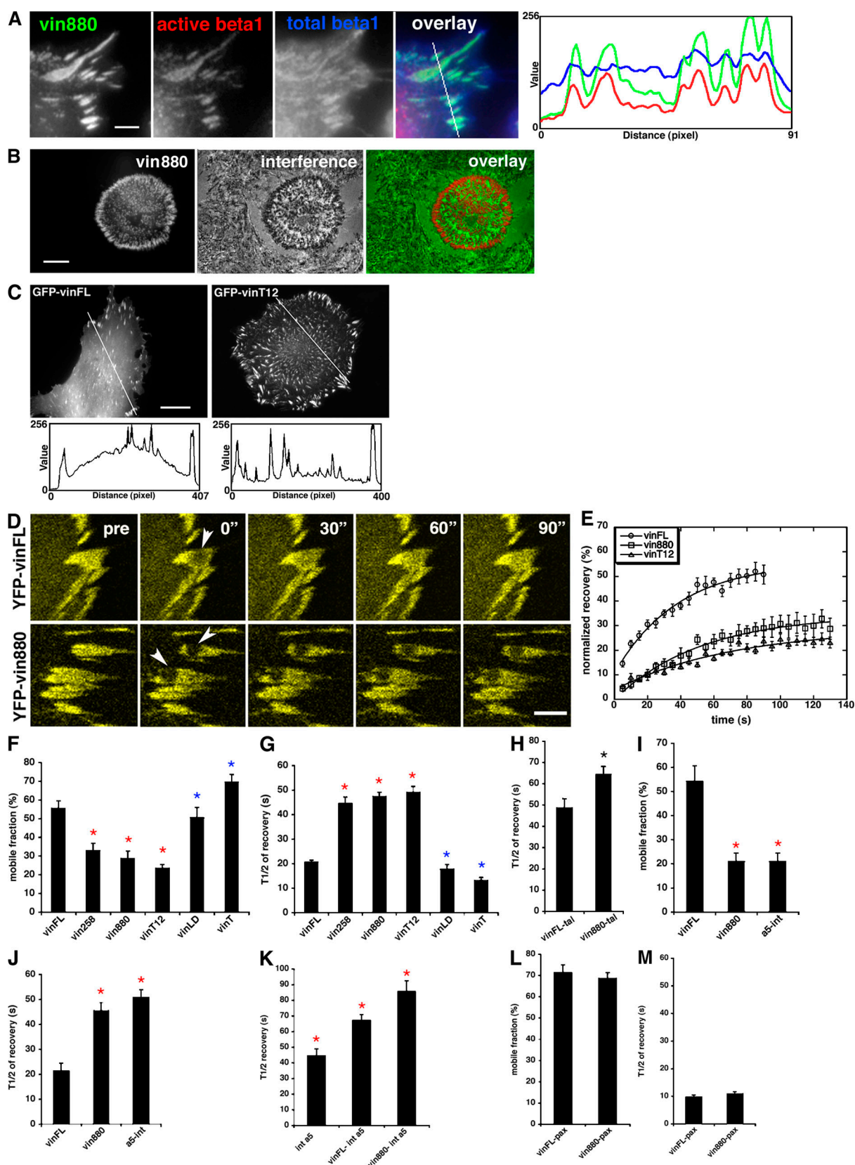
Figure 3. Vinculin regulates integrin clustering and dynamics. (A) HeLa cells overexpressing YFP-vin880 were costained with an antibody recognizing active \beta 1 (9EG7; Bazzoni et al., 1995) and the total pool of \beta 1 integrin (TS2/16). FAs positive for YFP-vin880 are also positive for \beta 1 integrins. The intensity profiles in red and green outline the high correlation of YFP-vin880 and active \beta 1 integrins. The blue intensity profile shows the high levels of \beta 1 integrins in the cell membrane and FAs. Fluorescence intensity profiles depict the area of the lines drawn in image overlays. (B) FAs induced by YFP-vin880 (left) are readily visible by interference reflection microscopy (middle), indicating that they participate in adhesion to ECM proteins. Overlay fluorescence and interference are shown on the right. (C) Images and line profiles drawn over the area of NIH3T3 cells expressing indicated constructs demonstrate that the cytoplasmic pool of
