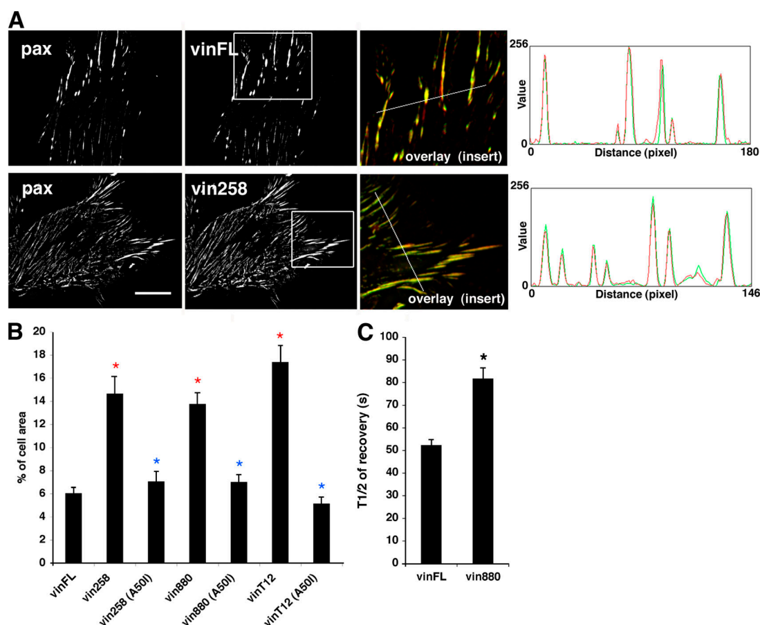
Figure 6. Vinculin-induced FA hypertrophy and paxillin recruitment to FAs is not due to the potential dimerization of tailless vinculin constructs with endogenous vinculin. (A) CFP-paxillin was coexpressed with YFP-vinFL or -vin258 in vin -/- MEF cells. Overlay images are from insert areas outlined in the vinFL and vin258 labeled images. The line profiles taken from the lines indicated on the left outline the nearly identical localization of the respective coexpressed proteins in FAs. Bar, 8 \mu m. (B) Quantification of FA sizes in vin -/- MEF cells expressing the indicated YFP fusion proteins. Area of FAs was calculated as a percentage of the total cell area. Red asterisks indicate significant differences of correlation values compared with vinFL ( P < 0.0001 , HSD test). Blue asterisks indicate no statistical differences to vinFL. (C) YFP-vin880 t_{1/2} of recovery is increased compared to YFP-vinFL when expressed in vin -/- MEF cells. Asterisk indicates statistical significance ( P < 0.001 , t test).
