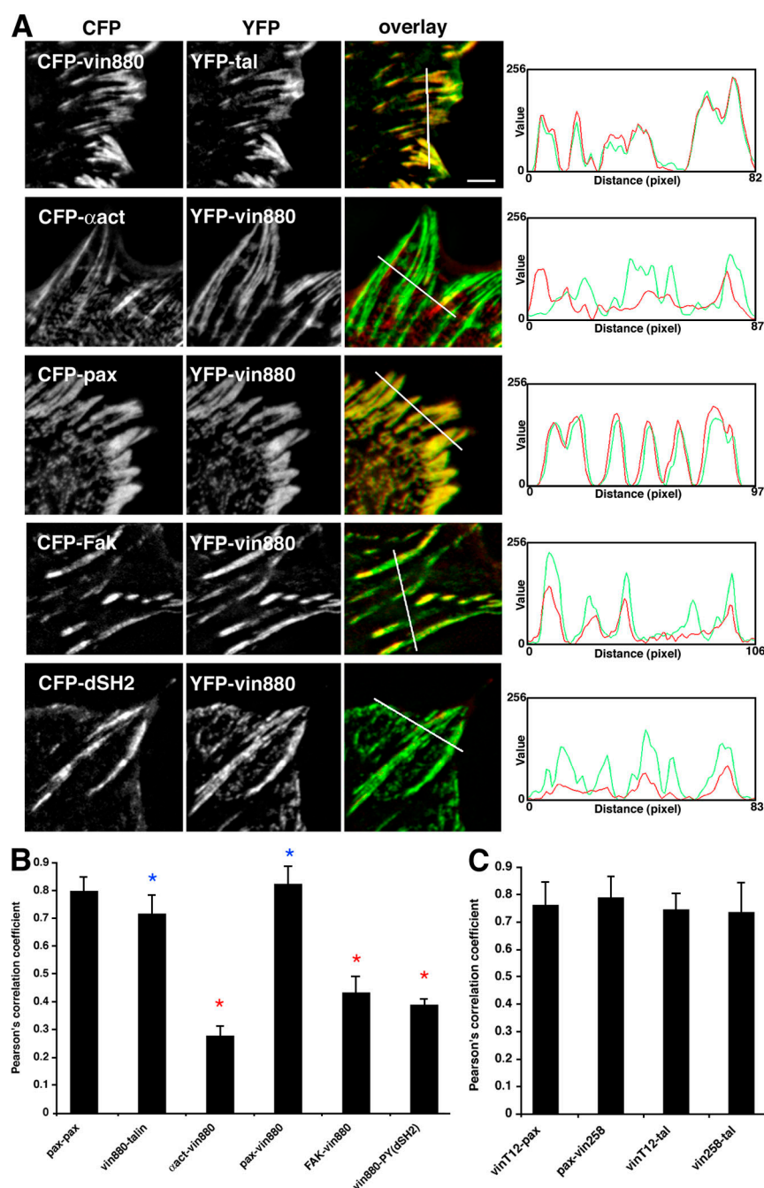
Figure 2. ICA of vin880 with other FA proteins.
