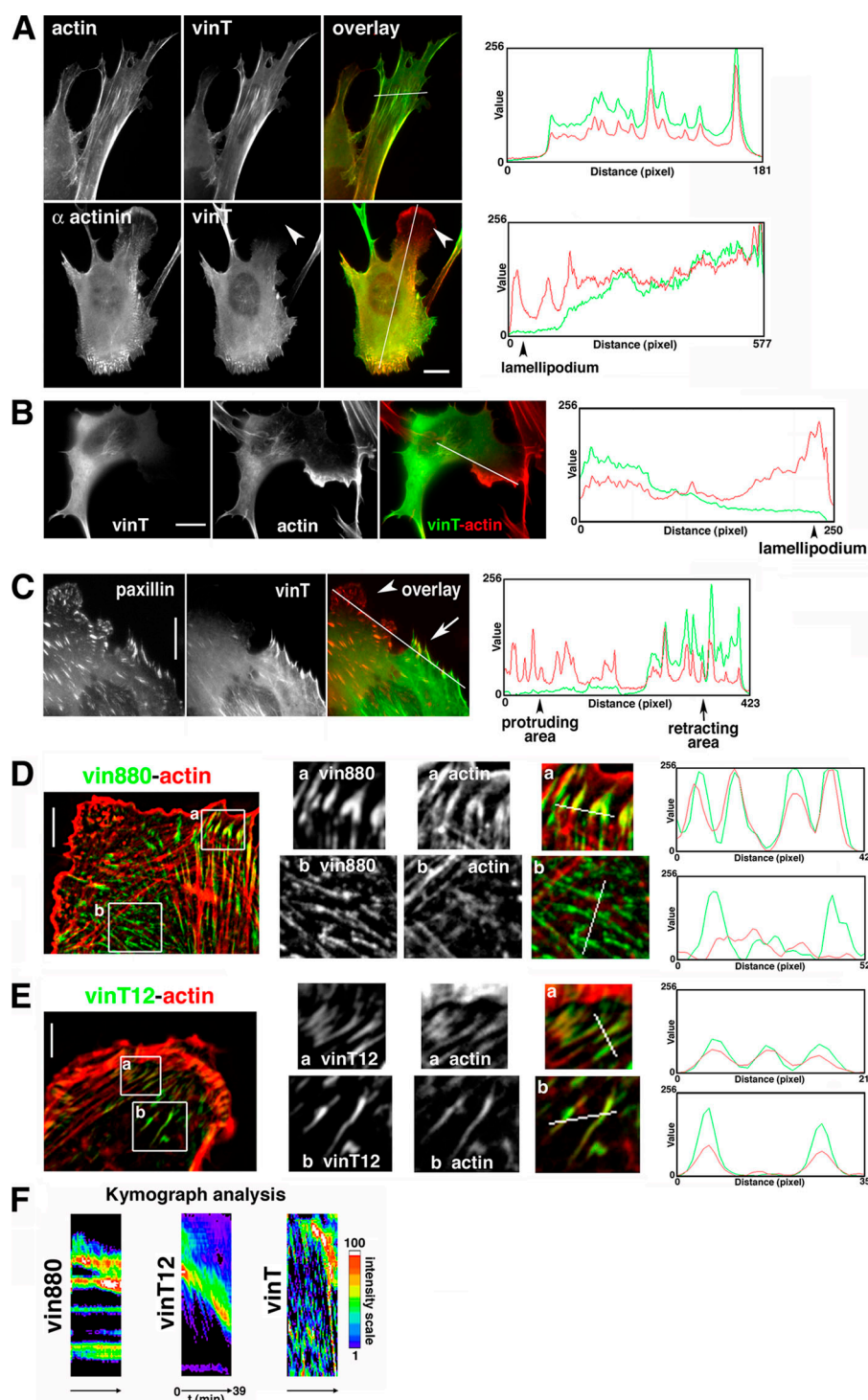
Figure 7. vinT colocalization correlates with a subset of actin but not paxillin. (A) Cells expressing vinT were either labeled for actin or cotransfected with CFP- \alpha -actinin (bottom). The intensity profiles on the right are from the area covered by the line in the overlay images. Note the high correlation of actin stress fibers with YFP-vinT. However, protrusive areas (white arrowheads) positive for \alpha -actinin remain free of YFP-vinT. Bar, 10 \mu m. (B) In vin -/- MEF cells, there is little YFP-vinT in protruding lamellipodia when compared to F-actin labeled with rhodamine-phalloidine. Note the strong correlation of the intensity profiles (right) on the left side and the lack of correlation on the right side (lamellipodium). (C) NIH3T3 cell expressing CFP-paxillin and YFP-vinT. The protruding area of cell shows many FAs in the protruding area positive for paxillin but devoid of vinT. To the right are line profiles of fluorescence intensities of the line in the overlay image (compare with Video 1, available at http://www.jcb.org/cgi/content/full/jcb.200703036/DC1 ). (D) NIH3T3 cell expressing YFP-vin880 and colabeled for actin. (a) FAs at the cell periphery with similar intensity profiles, indicating that these FAs are linked to actin stress fibers. (b) FAs away from the periphery of the cell. Intensity profiles show that intensity peaks of vin880 do not correlate with the actin intensities. (E) NIH3T3 cell expressing vinT12 and colabeled for actin. Intensity profiles taken from lines in inserts of peripheral and inner FA demonstrate a significant overlap of vinT12 and actin fluorescence intensity peaks, suggesting a link of these FAs with the actin cytoskeleton. (F) Kymograph analysis of NIH3T3 cells expressing YFP-vin880, GFP-vinT12, and YFP-vinT. Kymograph analysis shown in a spectral fluorescence intensity scale derived from a one-pixel line perpendicular to the cell edge of time-lapse recordings presented in Videos 2–4. Note that high intensity areas in vin880 cells remain stable with time and therefore are visualized as straight lines in this type of analysis, whereas those of vinT12 and vinT follow a retrograde flow. Bars (A–C) 10 \mu m; (D and E) 8 \mu m.
