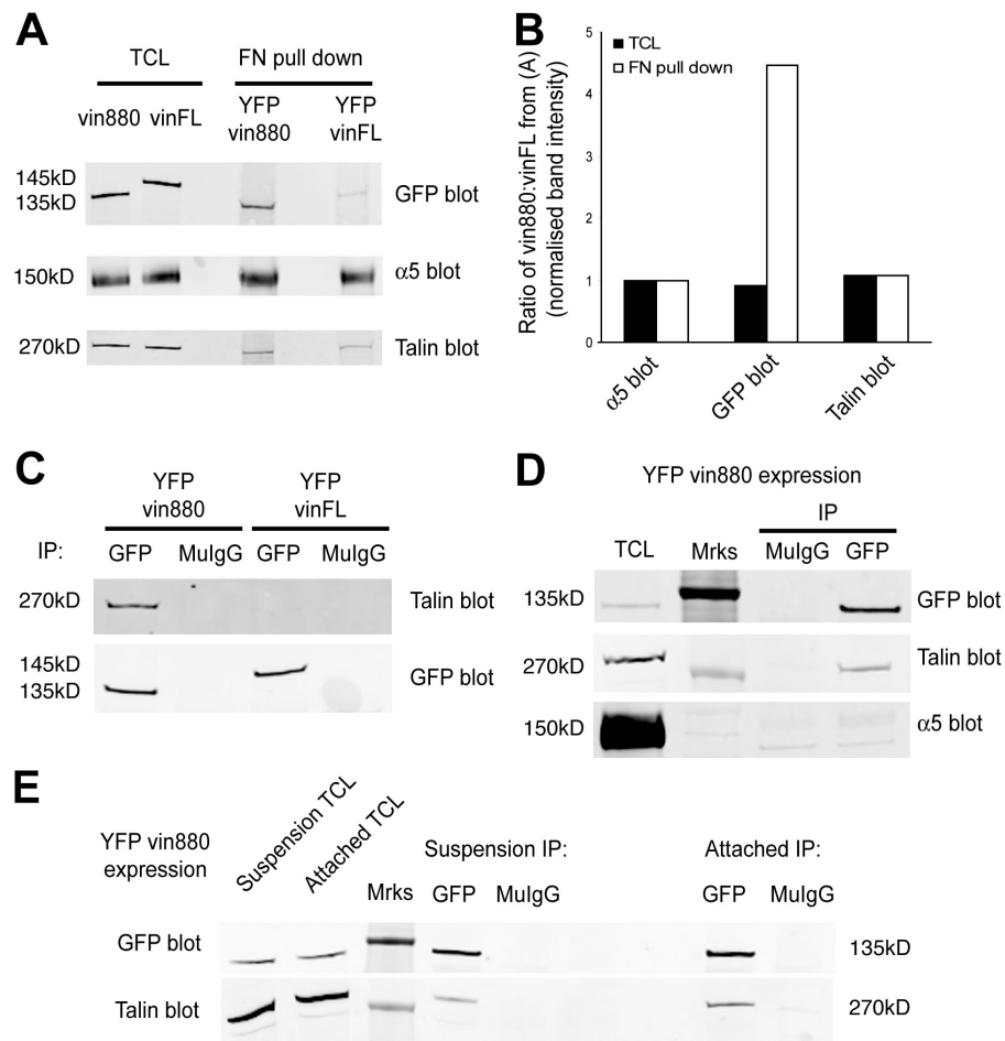
Figure 4. YFP-vin880 is enriched in FN-integrin complexes and coimmunoprecipitates talin and integrin. (A) FN-bead bound complexes isolated from NIH3T3 cells expressing either YFP-vin880 or -vinFL and immunoblotted for GFP, \alpha 5 integrin, or talin. (B) Quantification of A expressed as a ratio of vin880/vinFL after immunoblot band signal intensity normalization to the respective \alpha 5 integrin signal intensity. Open bars represent ratios of indicated proteins from pull-down experiments with pFN-coated beads; shaded bars represent protein ratios detected in total cell lysate (TCL) of cells expressing YFP-vin880 or -vinFL. (C) Immunoprecipitations using anti-GFP or control mouse IgG (MulgG) from NIH3T3 cells expressing either YFP-vin880 or -vinFL. (D and E) Immunoprecipitations using anti-GFP or control MulgG from NIH3T3 cells expressing YFP-vin880 after treatment with a chemical cross-linker (D) or from cells in suspension for 15 min (E) versus cells left attached to tissue culture dishes. All blots are representative of more than two independent transfections. Mrks denotes the position of molecular mass standards (250 kD for talin blots and 150 kD for GFP and \alpha 5 integrin blots), which are visible by Western blotting using the infrared imaging system.
