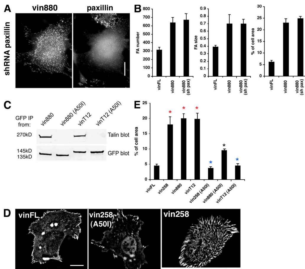
Figure 5. FA size is regulated by vinculin interaction with talin. (A) Paxillin was knocked-down using small hairpin RNA in B16 melanoma cells expressing vin880. Despite the absence of paxillin, vin880 still induced FA growth. (B) Quantification of FA number, size, and area fraction of indicated constructs in B16 cells with or without (sh pax) paxillin. (C) Immunoprecipitations from cell lysates of HeLa cells expressing either YFP-vin880, -vin880 (A50I), -vinT12, or -vinT12 (A50I) with anti-GFP antibodies. Note talin coimmunoprecipitates with vin880 and vinT12 but not with A50I mutants. (D) NIH3T3 cells expressing YFP-vinFL and -vin258 (A50I) show no significant differences in FA size in contrast to cells expressing YFP-vin258. (E) Quantification of FA size of cells expressing indicated constructs. Area of FAs was calculated as a percentage of the total cell area. Red asterisks indicate significant differences compared with vinFL ( P < 0.0001 , HSD test). Blue asterisks indicate no statistical differences. Black asterisk indicates statistical difference with vinFL ( P < 0.001 , t test). Error bars indicate \pm SEM. Bars: (A) 10 \mu m; (D) 10 \mu m.
