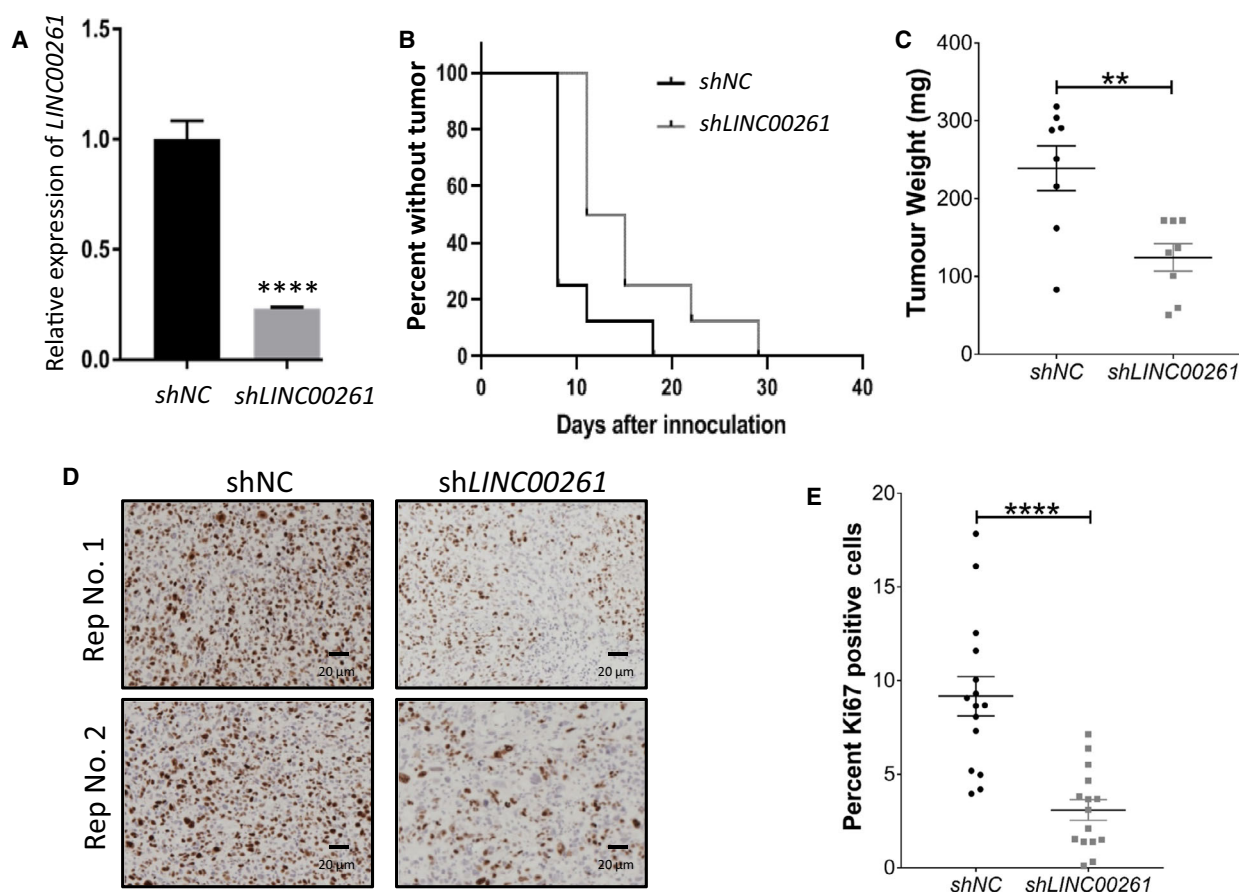
Fig. 3. LINC00261 silencing in vivo delays tumor formation. (A) LINC00261 expression (qPCR) in PC-3 cells stably expressing a non-targeting control ( shControl ) or shRNA targeting LINC00261 ( P < 0.0001 ). (B) Kaplan–Meier analysis for tumor formation in mice injected with cancer cells expressing shLINC00261 or shControl . (C) Tumor weight of control or LINC00261 -silenced PC-3 tumors upon harvest at day 32 after implantation into mice (** P = 0.0043 ). (D) Representative IHC images and (E) quantification of PC-3 tumors from the control or LINC00261 -silenced arms stained for the proliferation marker Ki67. The scale bar at the bottom marks a 20 μm width. (A, C) Analyzed by unpaired two-tailed t -test. (B) Analyzed by log-rank test: P = 0.018 . (E) Images analyzed using IMAGEJ (see Materials and methods); statistically analyzed by unpaired two-tailed t -test n = 15 . All data are presented as mean \pm SEM with at least three independent biological replicates. **** P < 0.001 .
