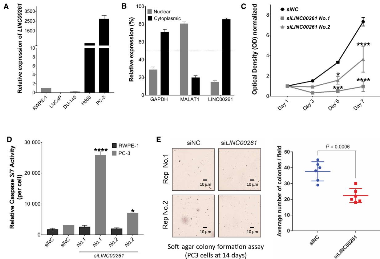
Fig. 2. LINC00261 is required for NEPC cell viability and invasiveness. (A) Expression (qPCR) of LINC00261 in a panel of prostate cell lines. (B) Subcellular localization of LINC00261 , GAPDH , and MALAT1 RNA transcripts in PC-3 cells. (C) Viability (MTT assay) of PC-3 cells treated with a control, nontargeting siRNA (siNC), or distinct siRNAs targeting LINC00261 at 10 nM dosage. (D) Cell viability-adjusted activity of caspase 3/7 after 72 h of siRNA-mediated LINC00261 knockdown in PC-3 cells. (E) Left, Representative images of iodinitrotetrazolium chloride stained soft agar PC-3 cell colonies after treatment with either the nontargeting, control siRNA (siNC), or siRNA targeting the LINC00261 (siLINC00261) transcript (two-tailed t -test). Right, Average number of soft agar colonies per 10x field of siNC- or siLINC00261-treated PC-3 cells. The scale bar at the bottom marks a 10 \mu m width. Distinct cells colonies were counted from three randomly chosen 10X field per well from two biological replicates. All data are presented as mean \pm SEM with at least two independent biological replicates. (C) Analyzed using two-way ANOVA with Tukey's multiple comparisons test. (D) Analyzed by one-way ANOVA with Dunnett's post hoc test. (E) Analyzed by two-tailed t -test. * P < 0.05 ; **** P < 0.001 .
