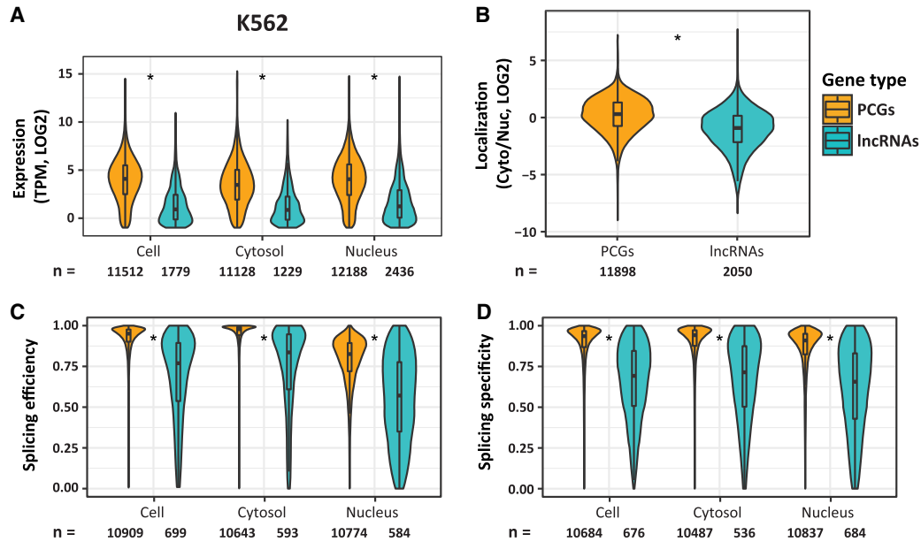
FIGURE 2. Differences between PCGs and lncRNAs in K562 cells. (A–D) Distributions of expression levels (A), Cyto/Nuc ratios (B), splicing efficiencies (C), and specificities (D), for PCGs and lncRNAs. (*) P -value < 10^{-16} (Wilcoxon rank sum test).
