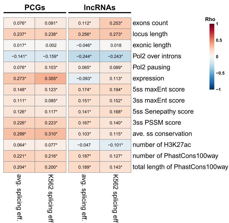
FIGURE 9. Factors associated with splicing efficiency. Correlation between the indicated features and splicing efficiency in PCGs and lncRNAs in K562 cells, or averaged across the nine cell lines (except for Pol2 occupancy, which is available in only six lines). Numbers indicate correlation coefficients. (*) P < 0.05 . Correlation coefficients and FDR-adjusted P -values computed using Spearman's correlation.
