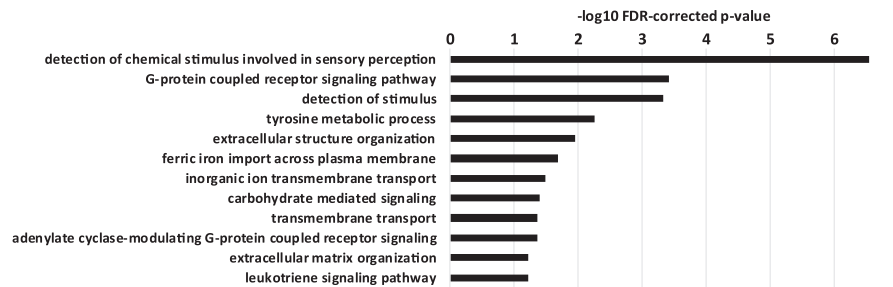
FIGURE 8. GO enrichment of nuclear-retained genes. GO analysis of ranked K562 Cyto/Nuc localization values. Bars indicate -\log_{10} FDR-corrected P-values for the respective GO-terms cluster (see Materials and Methods).
