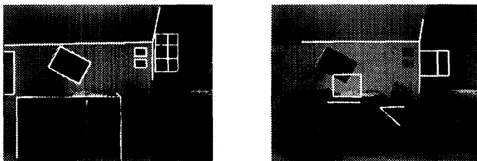
Fig. 4. Matching a model of office A to an image of office A (left), and matching a model of office B to the same image (right).
