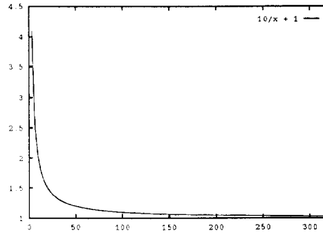
Fig. A.1. Z/Z_0 as a function of x for \epsilon = 10 pixels.
