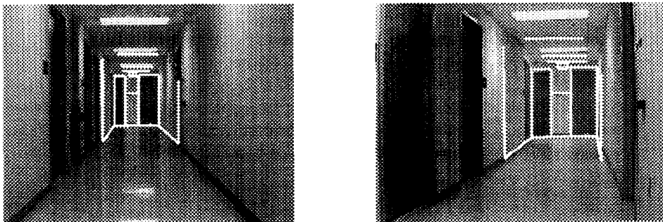
Fig. 10. Matching the corridor model with two images of the corridor. The right image was obtained by a relatively large motion forward (about half of the corridor length) and to the right. Note that the results of alignment when the picture is taken roughly under the conditions of Eq. (34) (left) are better than when these conditions are violated (right).
