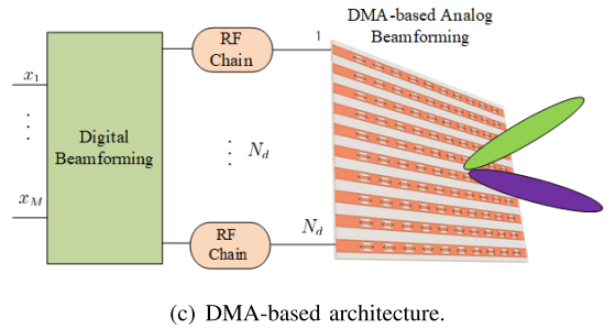
Fig. 3. Three typical antenna architectures.
