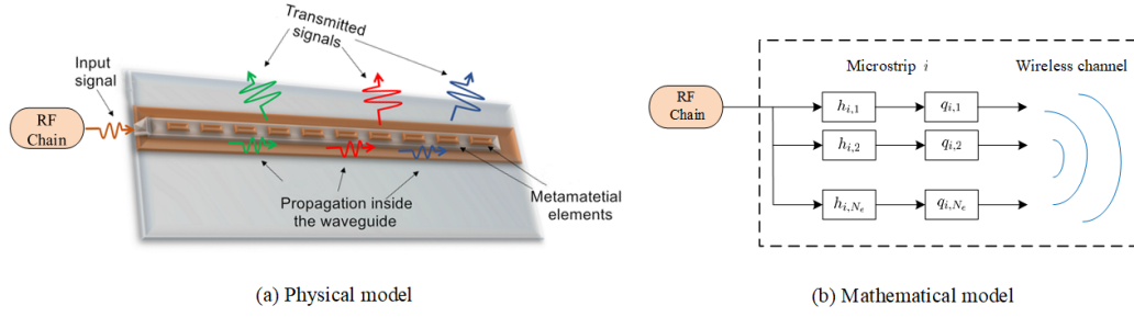
Fig. 4. Illustration of signal transmission using a microstrip. (a) Physical model; (b) Mathematical model.
