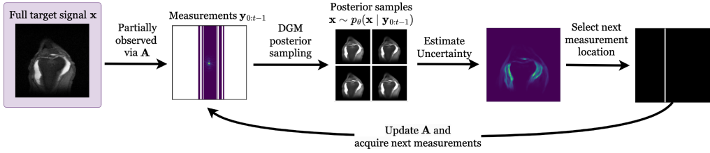
Figure 5. Illustrative example of an active CS step for MRI acceleration. The sensing matrix \mathbf{A} = \mathbf{U}\mathbf{F} consists of a subsampling matrix \mathbf{U} and DFT matrix \mathbf{F} . See fastMRI [1] for more information about MRI acceleration.
