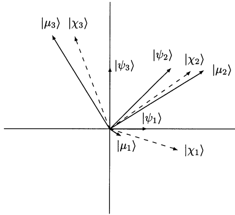
Fig. 1. Illustration of the optimal measurement vectors. The weighted state vectors are |\psi_i\rangle = \sqrt{p_i} |\phi_i\rangle where the vectors |\phi_i\rangle and the probabilities p_i are given by (34) and (35), respectively. The optimal measurement vectors |\mu_i\rangle are given by (40). The least-squares measurement vectors |\chi_i\rangle are plotted in dashed lines for comparison, and are given by (42).
