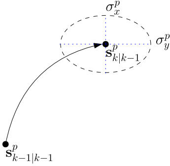
Fig. 5. Generation of the weighting matrix \mathbf{W}_k [as described in (10) and (11)]. Previously estimated state \mathbf{s}_{k-1|k-1}^p is propagated to state \mathbf{s}_{k|k-1}^p , according to (7). Its propagated error covariance matrix \mathbf{P}_{k|k-1}^p is then used to draw an ellipse around its location, where \sigma_x^p = \mathbf{P}_{k|k-1}^p[1, 1] and \sigma_y^p = \mathbf{P}_{k|k-1}^p[3, 3] . Aggregation of all propagated uncertainty ellipses generates an image of possible MBs locations. The matrix \mathbf{W}_k is proportional to the inverse of this image.
