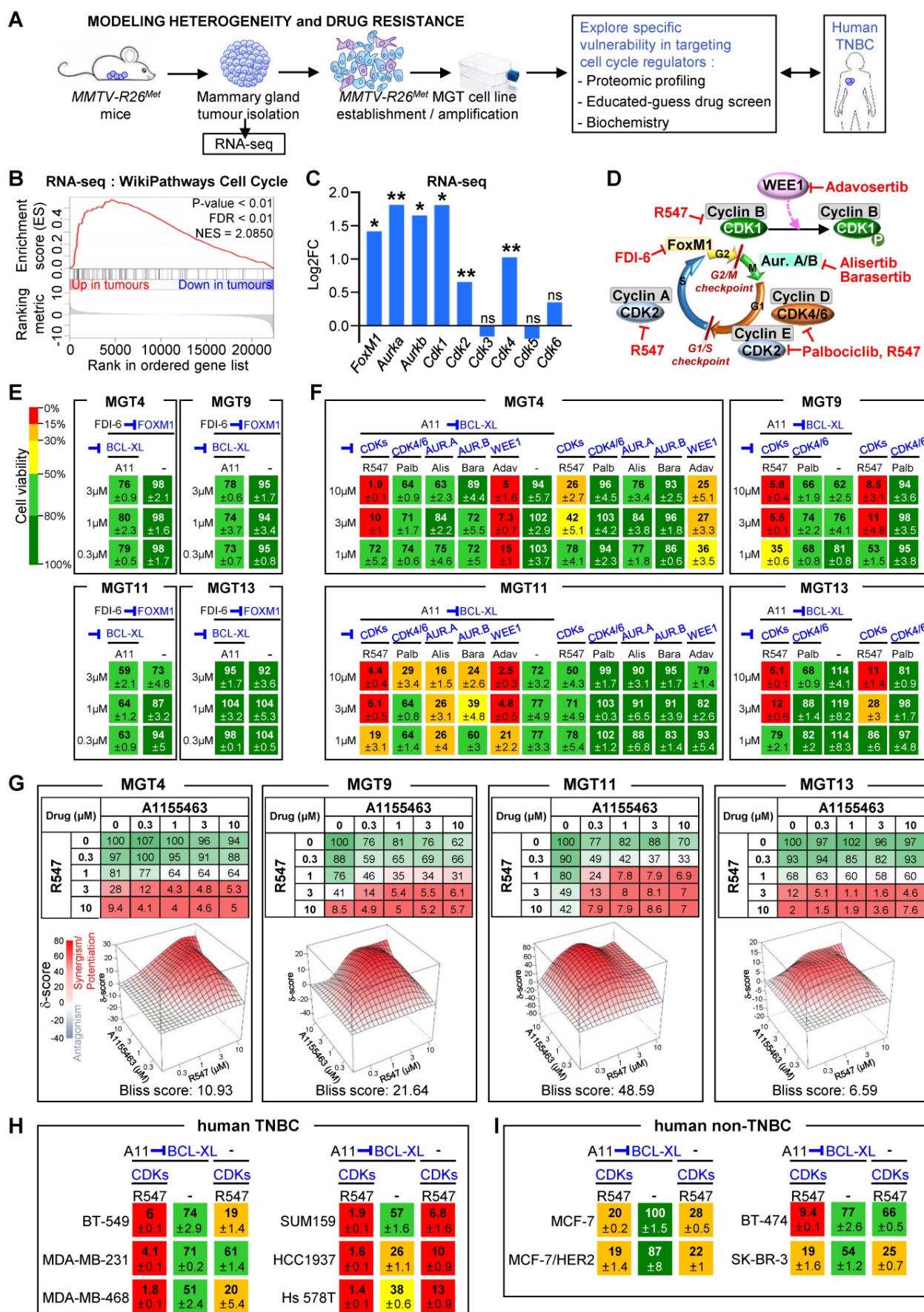
Figure 3. Combined inhibition of BCL-XL and CDK1/2/4 is deleterious for MMTV-R26 Met and human TNBC cell lines. (A) Scheme illustrating the strategy used in this study to explore the vulnerability of TNBC cells to the inhibition of specific cell cycle regulators in combination with BCL-XL targeting. RNA-seq studies were performed
