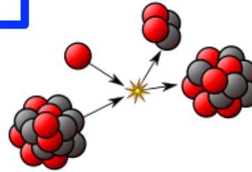
Nuclear Fision by a neutron
