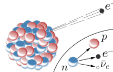
Radioactive decay And proton emission, Beta particl (electron) And Gamma radiation.
