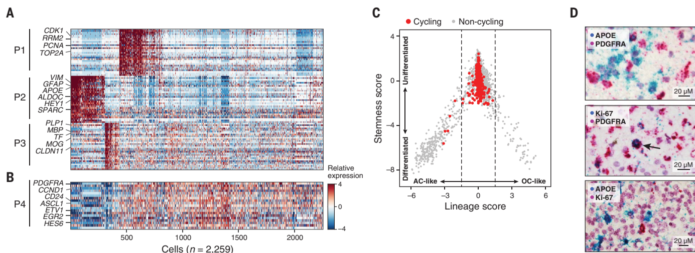
Fig. 2. Intratumor heterogeneity in H3K27M-glioma. (A and B) Relative expression (color bar) across 2259 malignant cells (columns) of the top 30 genes for each of the combined expression programs P1, P2, and P3 [(A), rows] or 19 genes [(B), P4] that are preferentially expressed in cells with low expression of P1, P2, and P3 (8). (C) Plot of the lineage
