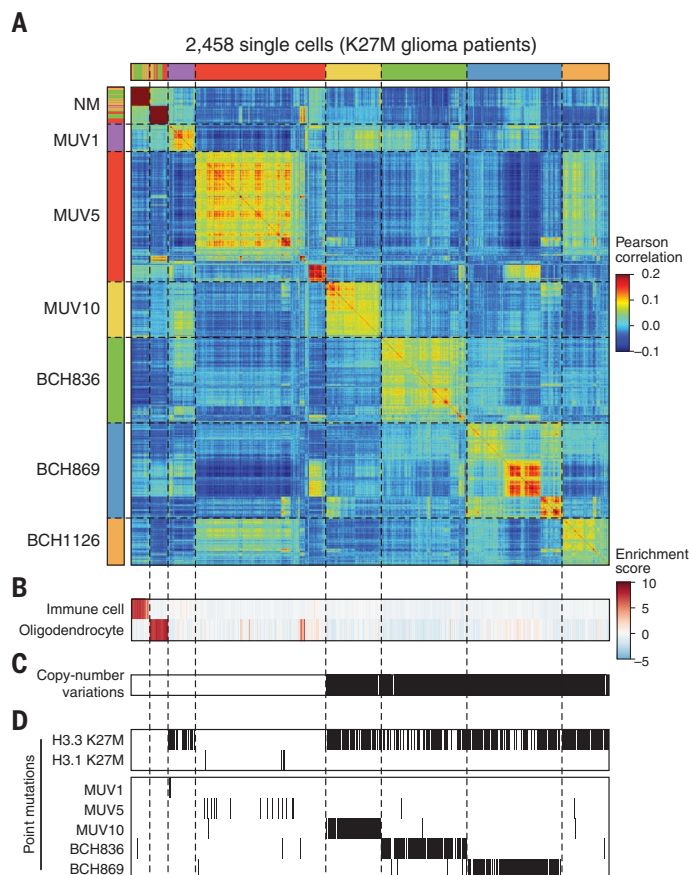
Fig. 1. Characterization of H3K27M-glioma by means of scRNA-seq. (A) Pair-wise correlations between the expression profiles of 2458 single cells (rows, column) from six H3K27M-glioma samples (color bar). Two clusters of nonmalignant cells are marked as "NM." (B) Enrichment score of microglia and oligodendrocyte signatures. (C) Inferred CNV profiles. Black indicates CNV present (fig. S4). (D) Gene mutations. (Top) H3K27M.; (Bottom) All other mutations identified per sample by means of WGS/WES. Black line indicates at least one mutated gene identified (fig. S6).
