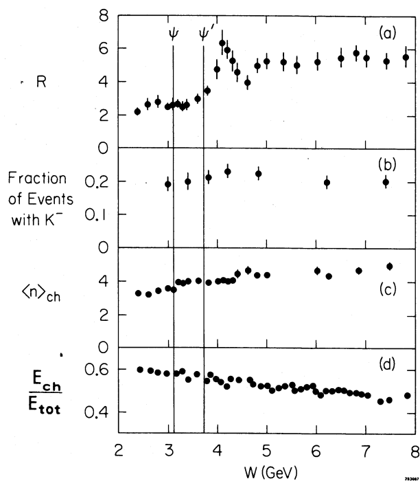
Fig. 7-- R , fraction of events with K^- , \langle n \rangle_{ch} , and E_{ch}/E_{tot} as a function of W .
