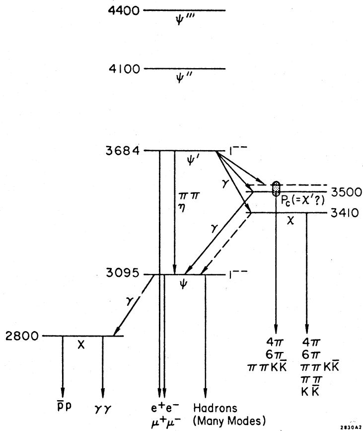
Figure 2: Present status of the \psi -spectrum.
