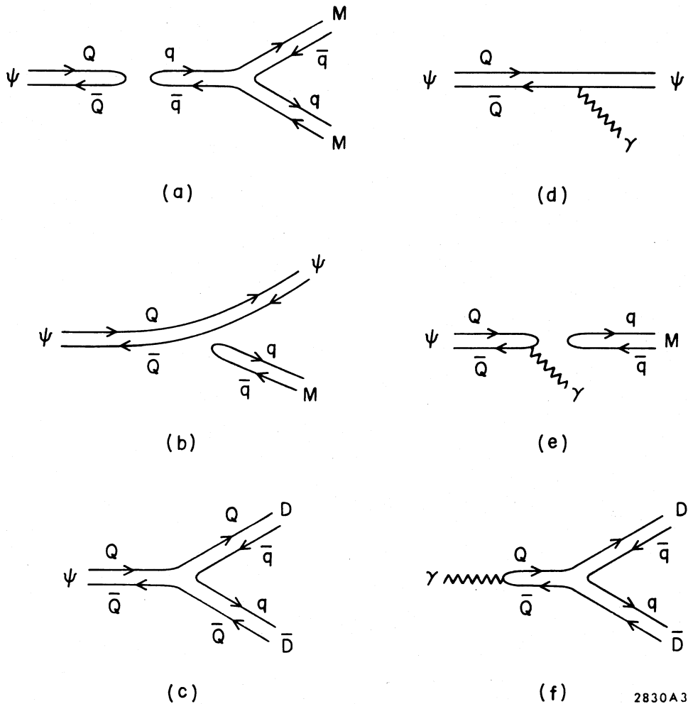
Figure 3: Quark diagrams for reactions involving M, D and \Psi mesons.
