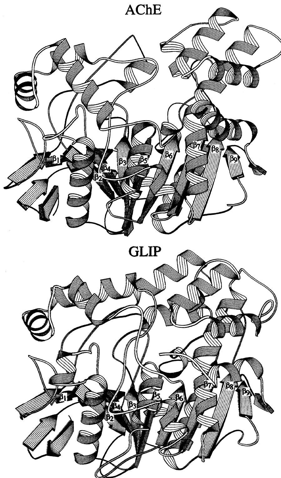
FIG. 2. Ribbon diagrams (18) of AcChoEase ( Upper ) and GLIP ( Lower ). \alpha -Helices are color-coded in red, and \beta -strands are in green. Both enzymes are in the same orientation. Strands of the central \beta -sheet are numbered sequentially ( \beta_0 – \beta_{10} ) in both enzymes following the scheme of the \alpha/\beta -hydrolase fold (19, 20). The active-site gorge of AcChoEase is located in the crevice between the \alpha -helices above strand \beta_5 .
