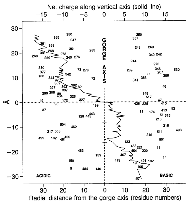
FIG. 3. Distribution of charged groups relative to the gorge axis in AcChoEase. Position of the gorge axis (i.e., the line approximating the center of the gorge) was determined visually with computer graphics and is represented by the middle vertical line (---). The horizontal axis (· · ·) represents a reference plane perpendicular to the gorge axis, at the level of the gorge bottom. This level is defined as the center of a 1.4-Å probe sphere at the point of its deepest possible penetration. Residue numbers indicate the relative positions of charged groups along the gorge axis (vertical scale) and their radial distance from the gorge axis (bottom horizontal scale). Acidic residues (aspartate, glutamate) are left of the gorge axis, and basic residues (lysine, arginine) are right of the axis. At each level along the gorge axis, the solid line (—) indicates the total cumulative charge between a plane perpendicular to the gorge axis at that level and the reference plane. The overall net charge on the enzyme, -8 electronic charges (e), is an algebraic sum of the net charge above (-17 e) and below (+9 e) the reference plane. The three acidic residues that are not resolved in the crystal structure would likely be located near the gorge axis at the bottom of the figure. There is clearly an unequal distribution of positive and negative charges in the two halves of the enzyme, giving rise to an overall net dipole. Note that only three negatively charged groups (residues 72, 199, and 285) are close enough to the gorge axis to interact directly with substrates in the gorge. The positions of several residue numbers were adjusted slightly for clarity.
