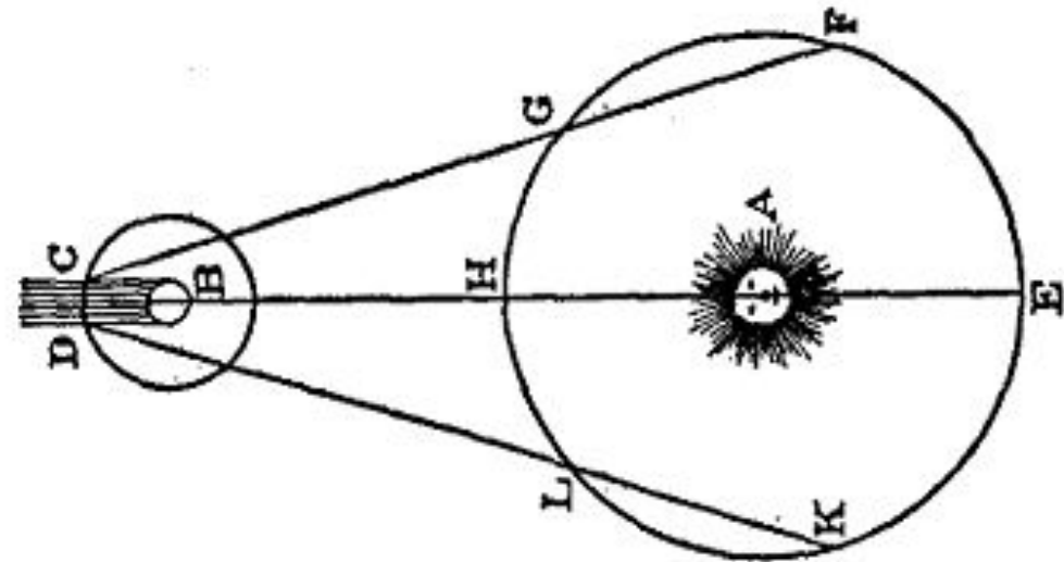
Velocity of light using Io orbit cycle.
