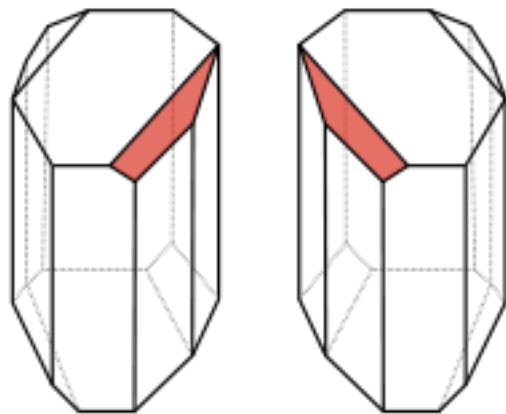
Tartaric acid enantiomers
